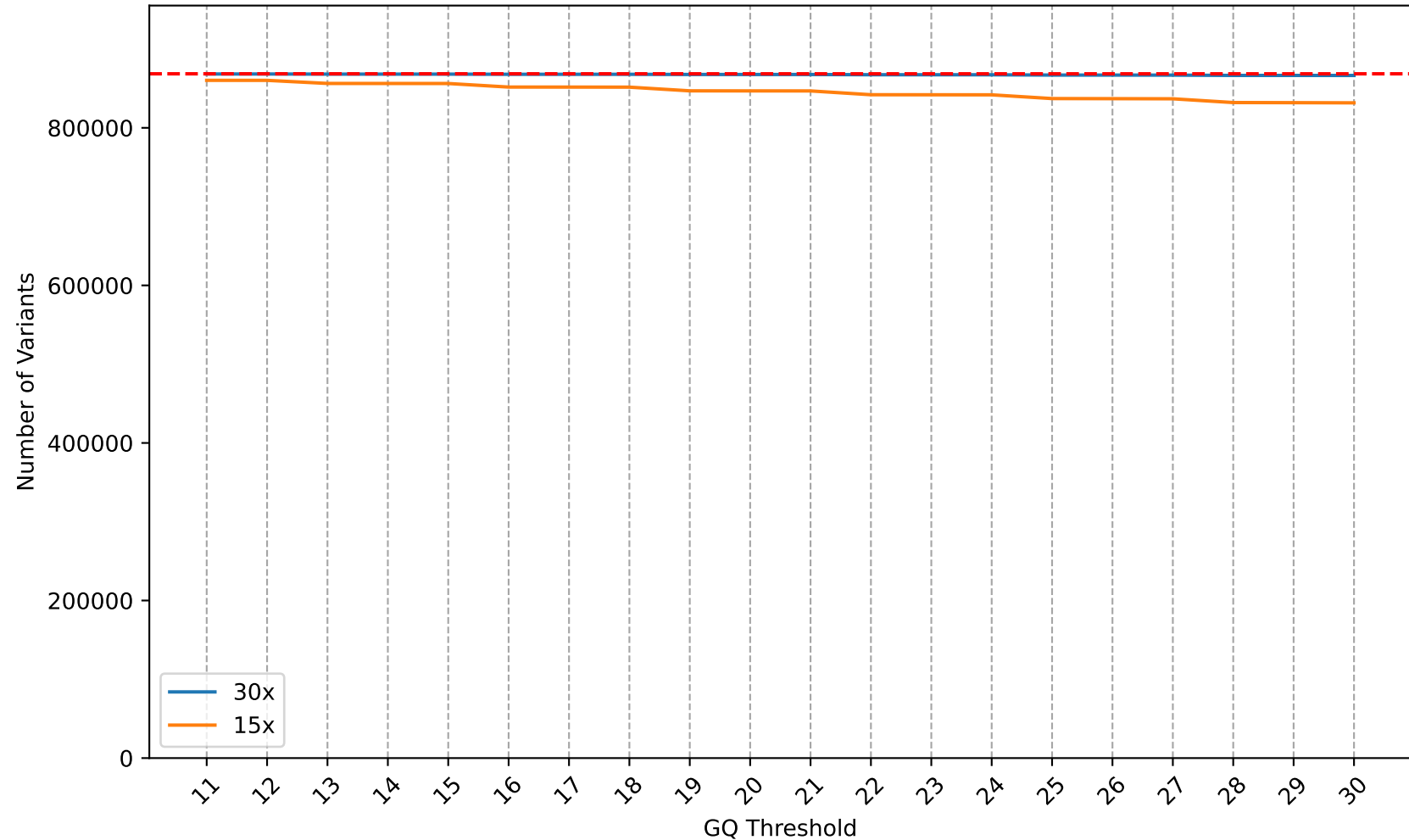
Remaining Variants Across GQ Thresholds (chr21)
