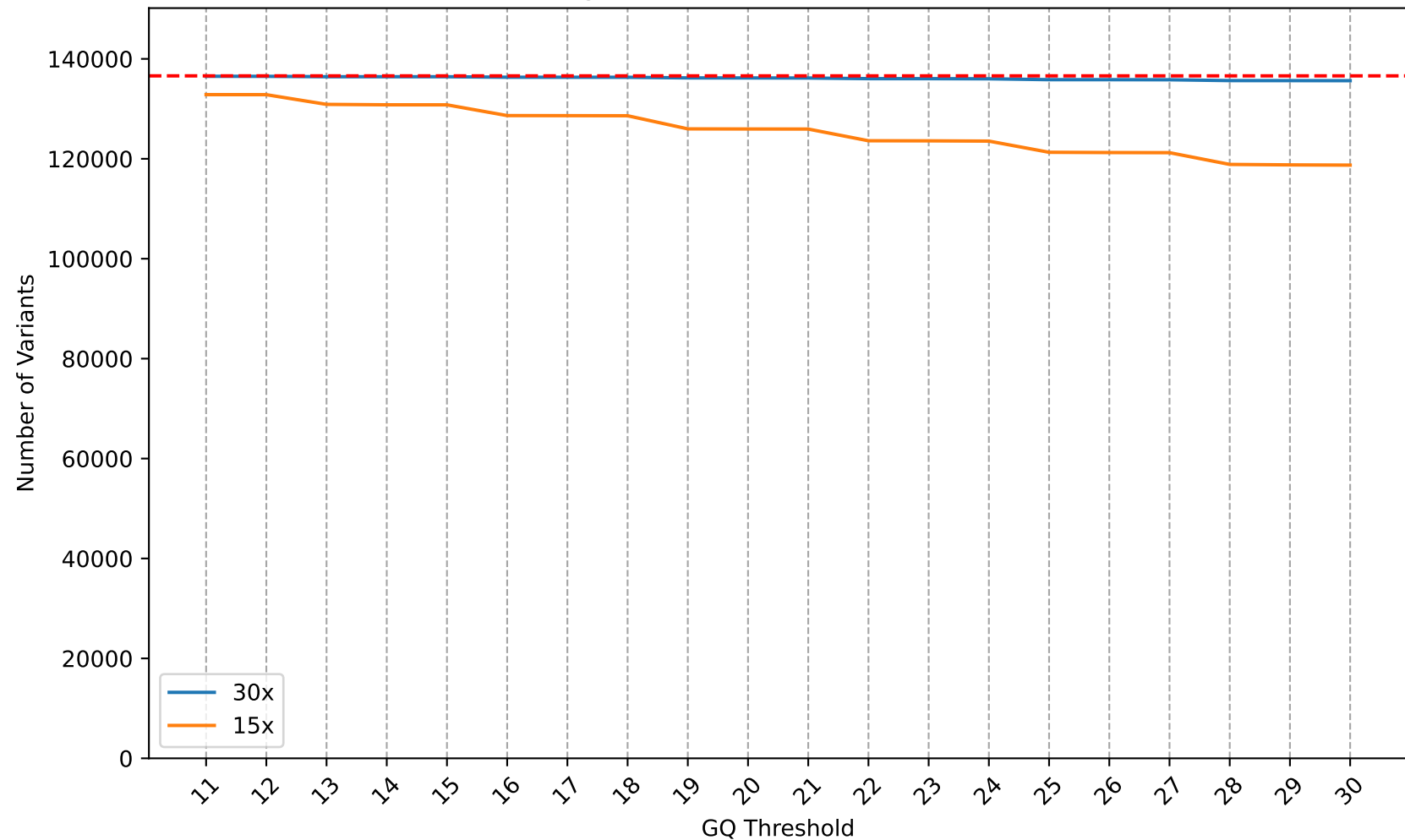
Remaining Variants Across GQ Thresholds (PAR)
