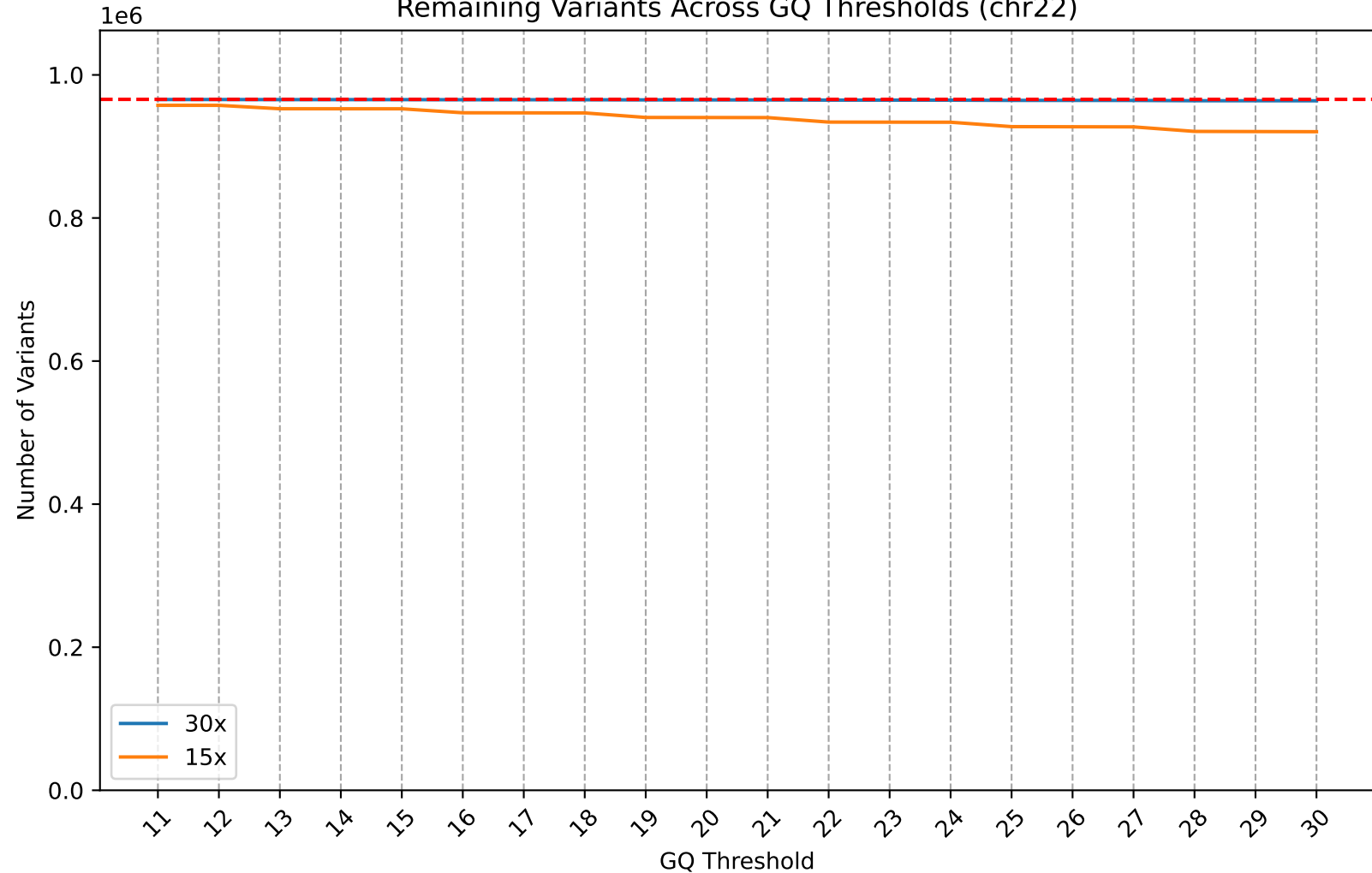
Remaining Variants Across GQ Thresholds (chr22)
