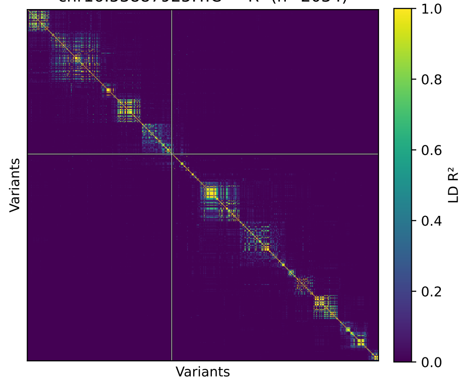
chr16:53887925:T:C — R 2 (n=2034)
