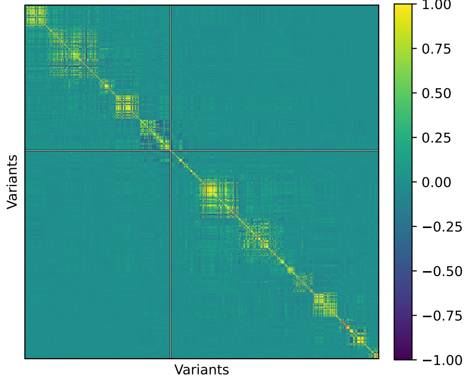
chr16:53887925:T:C — R (n=2034)
