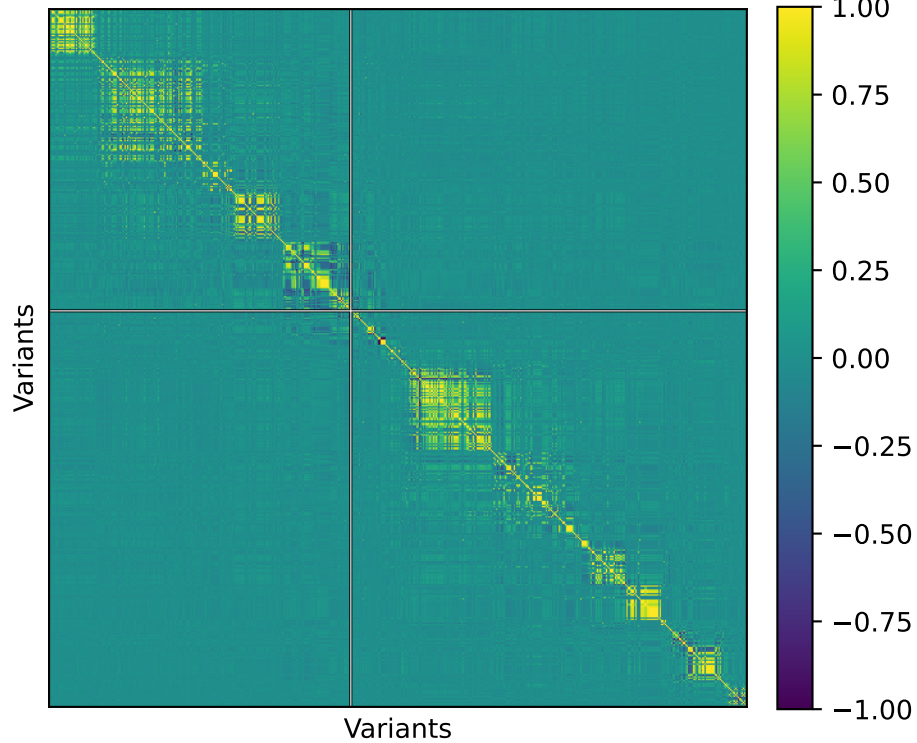
chr16:53887925:T:C — R (n=2182)
