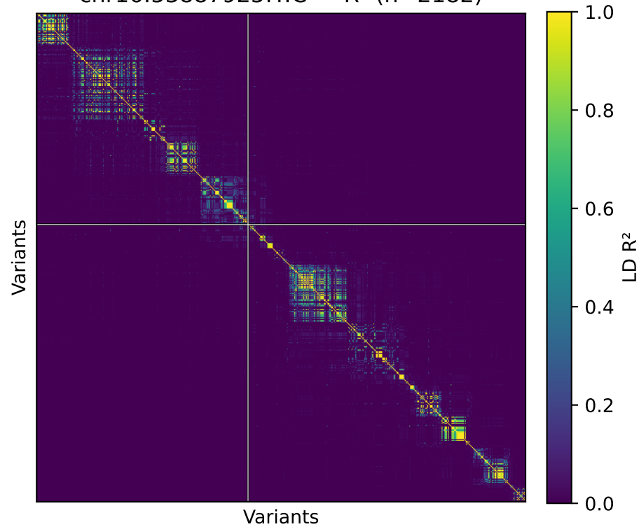
chr16:53887925:T:C — R 2 (n=2182)
