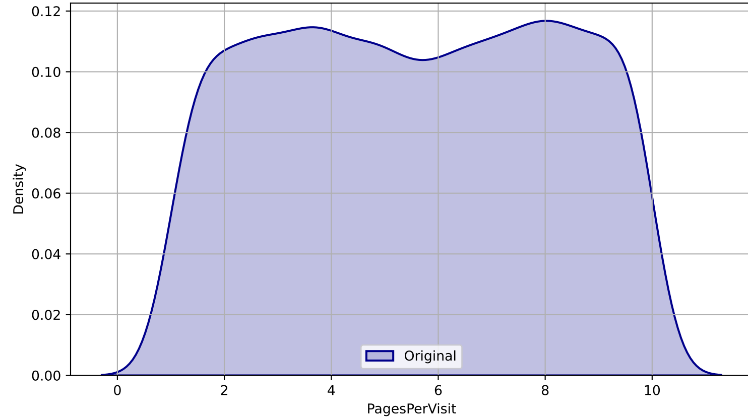
Original Density Plot for PagesPerVisit
