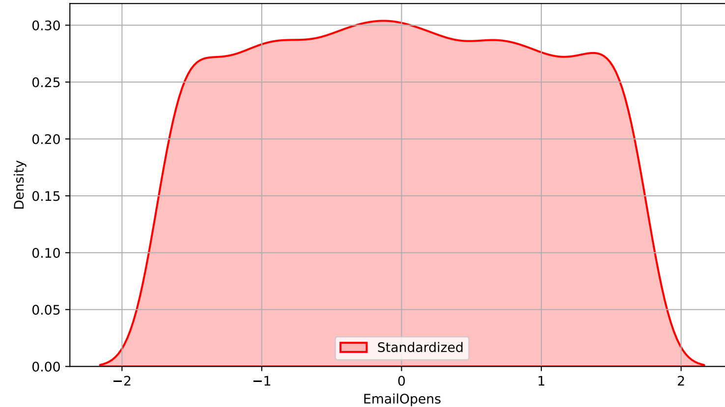
Standardized Density Plot for EmailOpens
