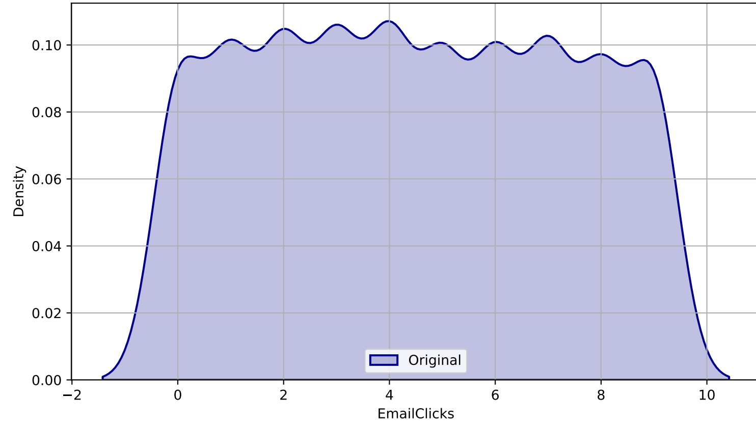
Original Density Plot for EmailClicks
