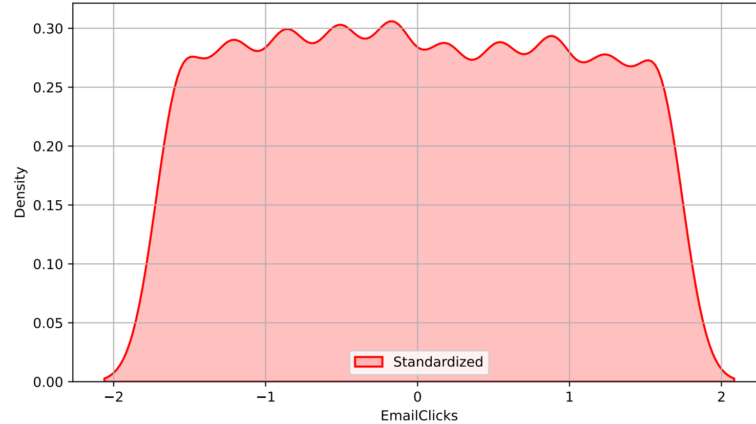
Standardized Density Plot for EmailClicks
