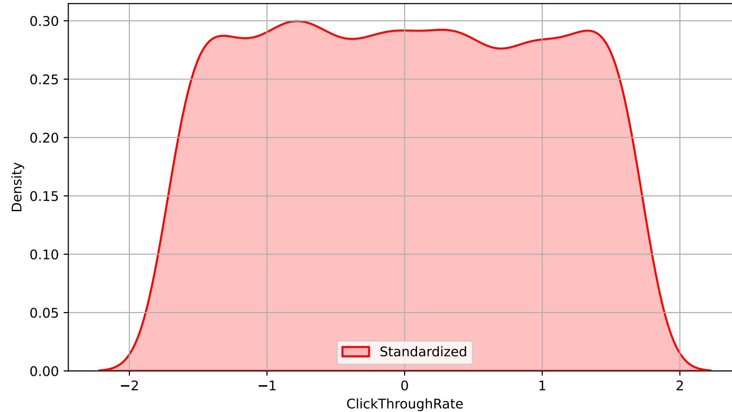
Standardized Density Plot for ClickThroughRate
