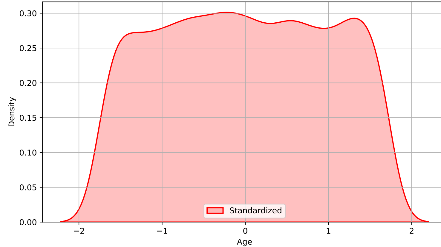
Standardized Density Plot for Age
