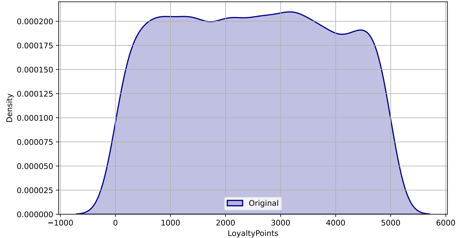
Original Density Plot for LoyaltyPoints
