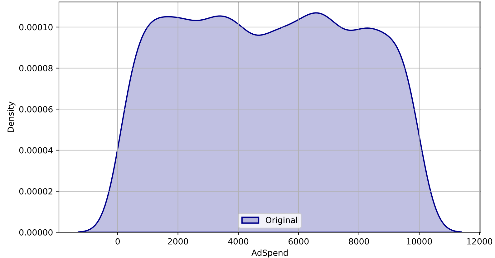
Original Density Plot for AdSpend
