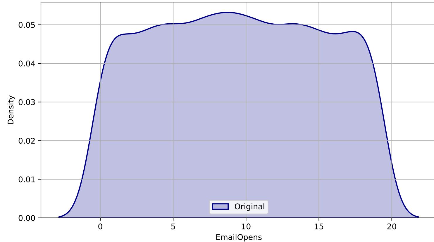
Original Density Plot for EmailOpens
