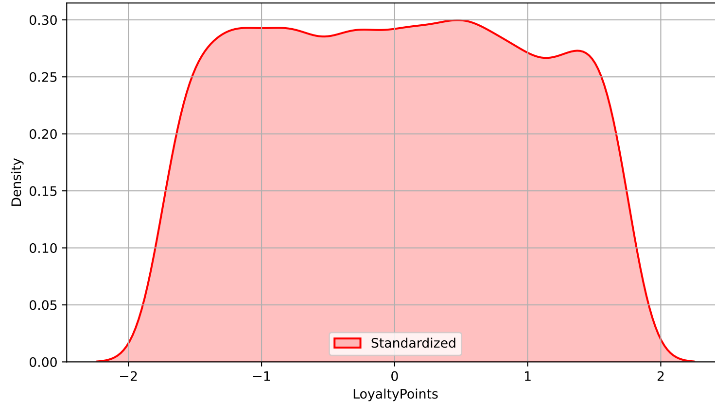
Standardized Density Plot for LoyaltyPoints
