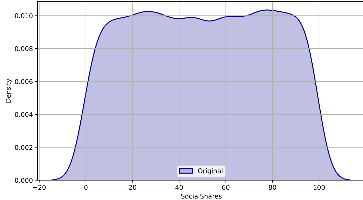
Original Density Plot for SocialShares
