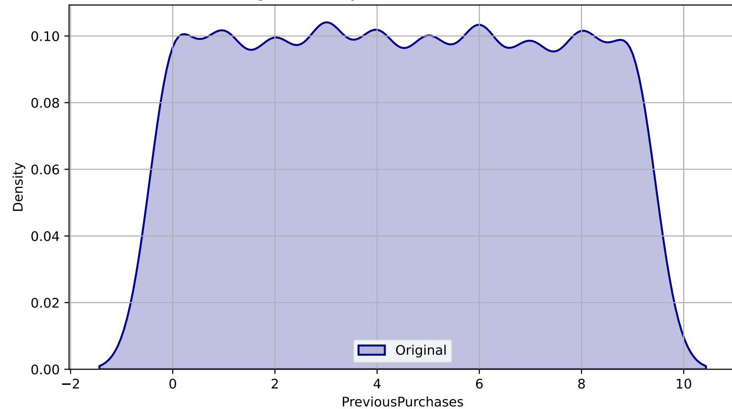
Original Density Plot for PreviousPurchases
