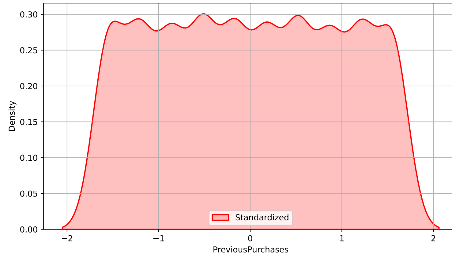
Standardized Density Plot for PreviousPurchases
