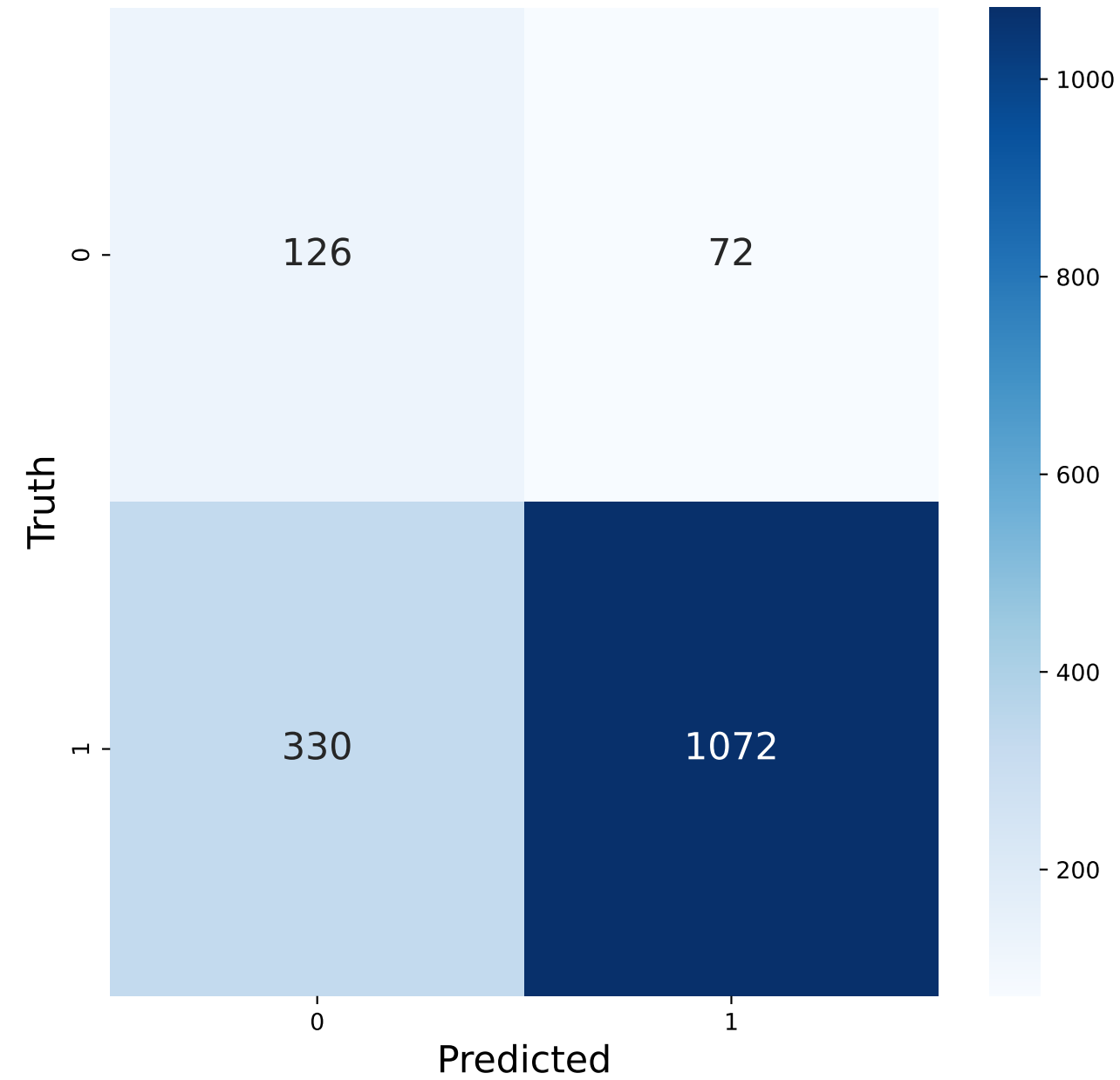
Confusion Matrix
