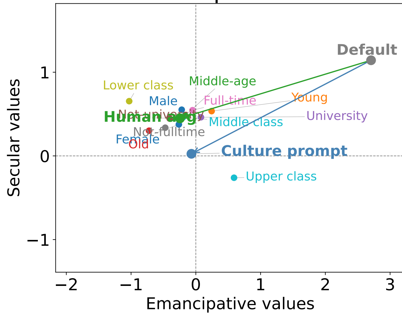
GPT | Serbia
