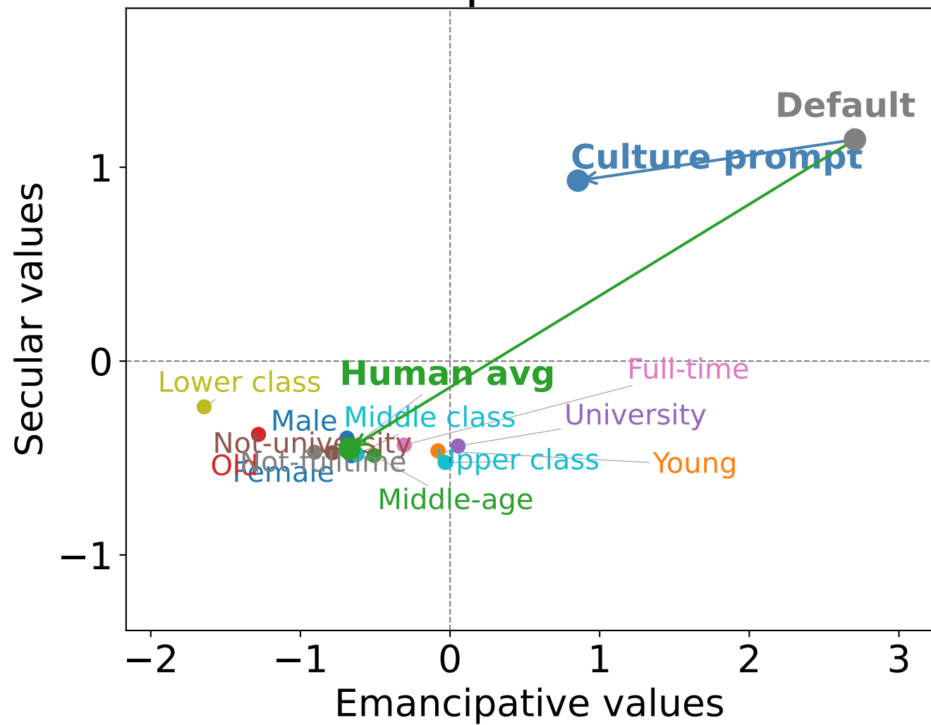
GPT | Greece
