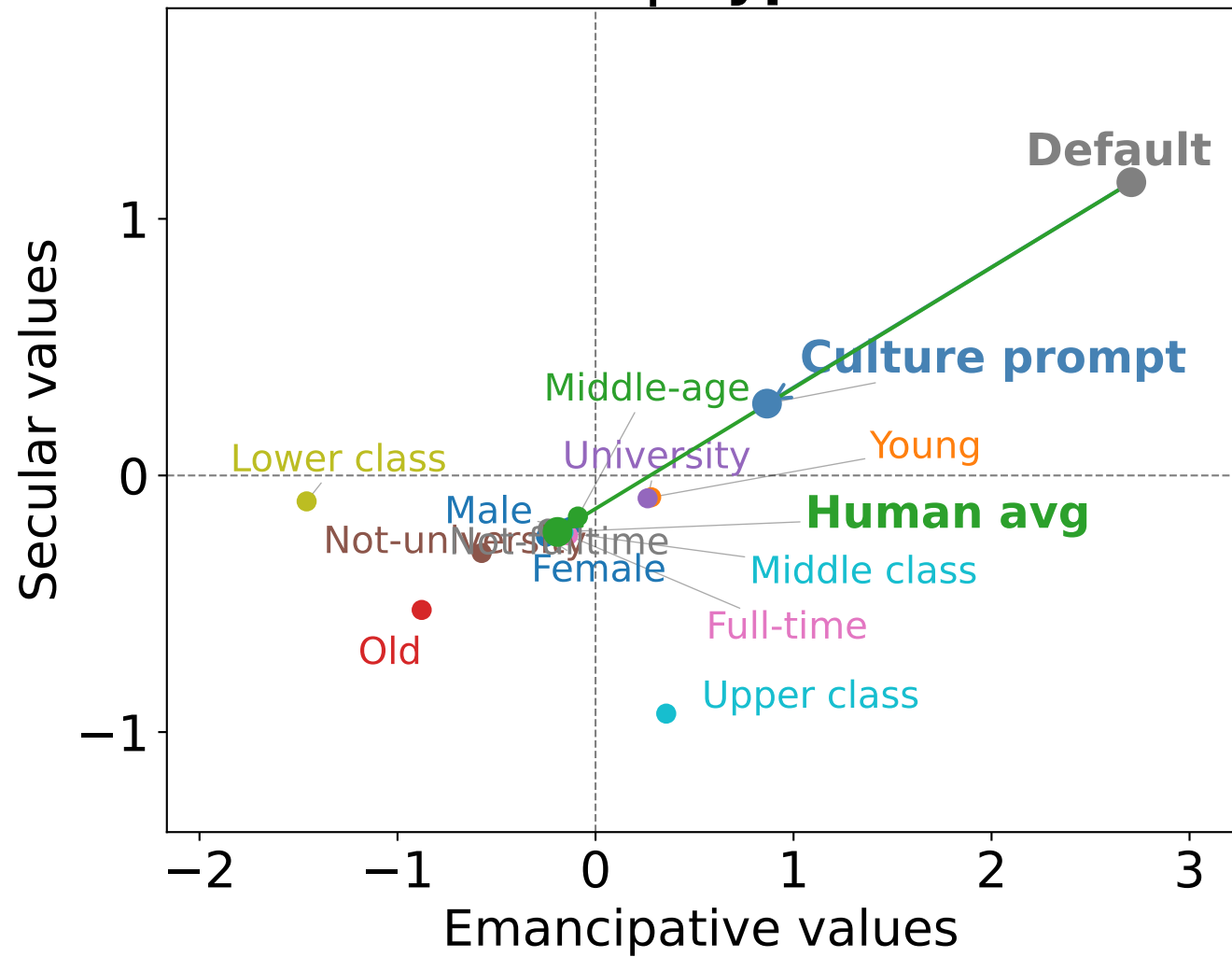
GPT | Cyprus
