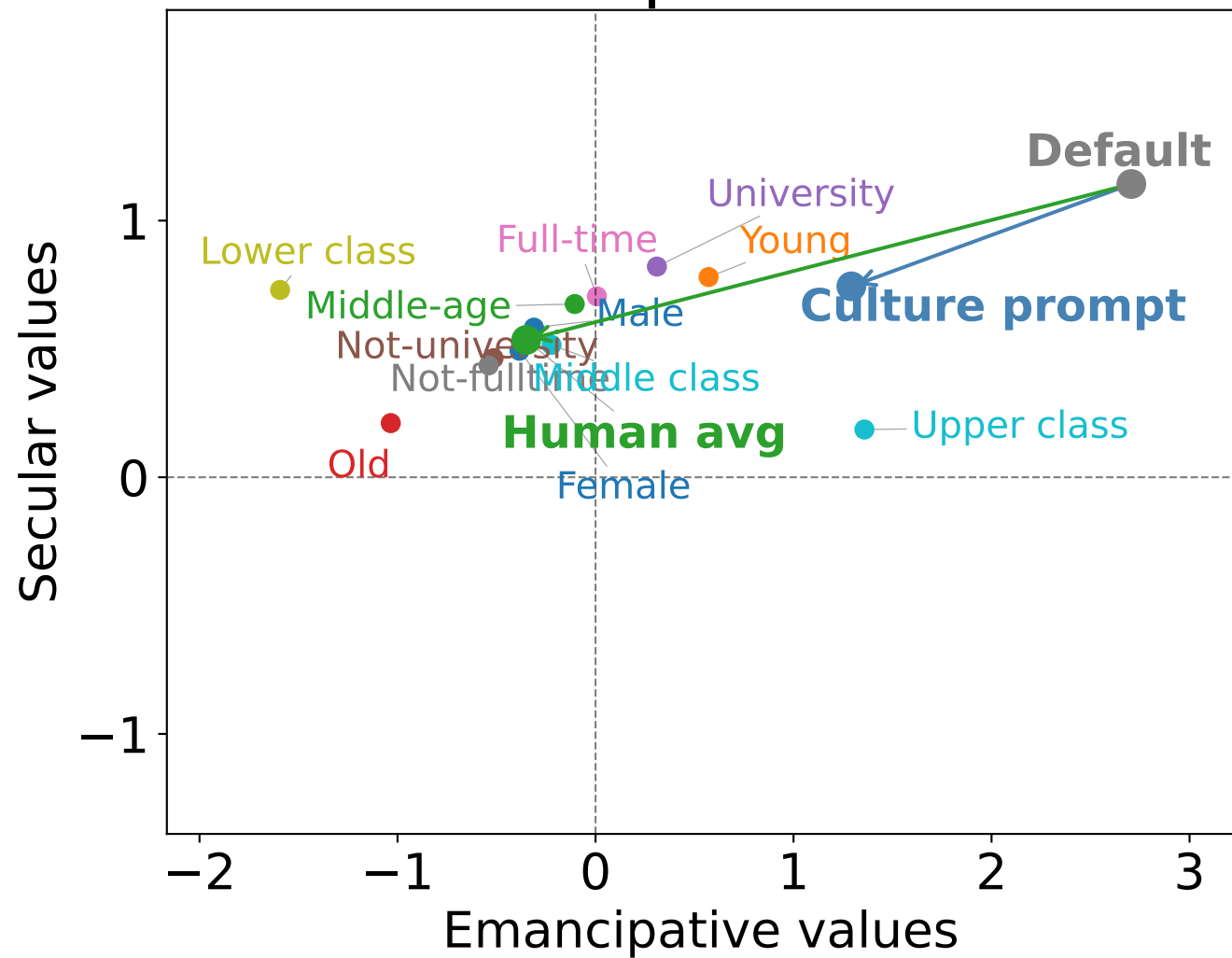
GPT | Cyprus
