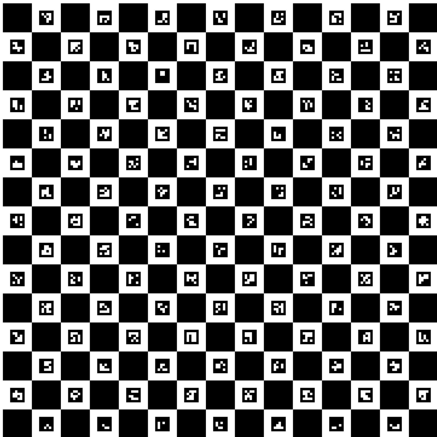
ChArUco Calibration Board Dictionary: DICT_4X4_250 Grid: 15 x 15 squares Square: 20.0 mm Marker: 10.0 mm Physical size: 300.0 x 300.0 mm Export DPI: 300
