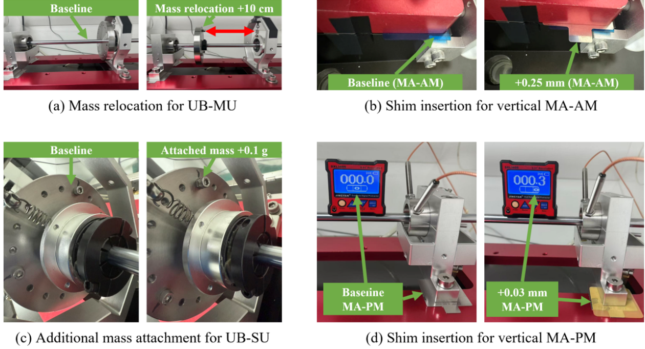
Figure 3: Representative fault-seeding operations.
