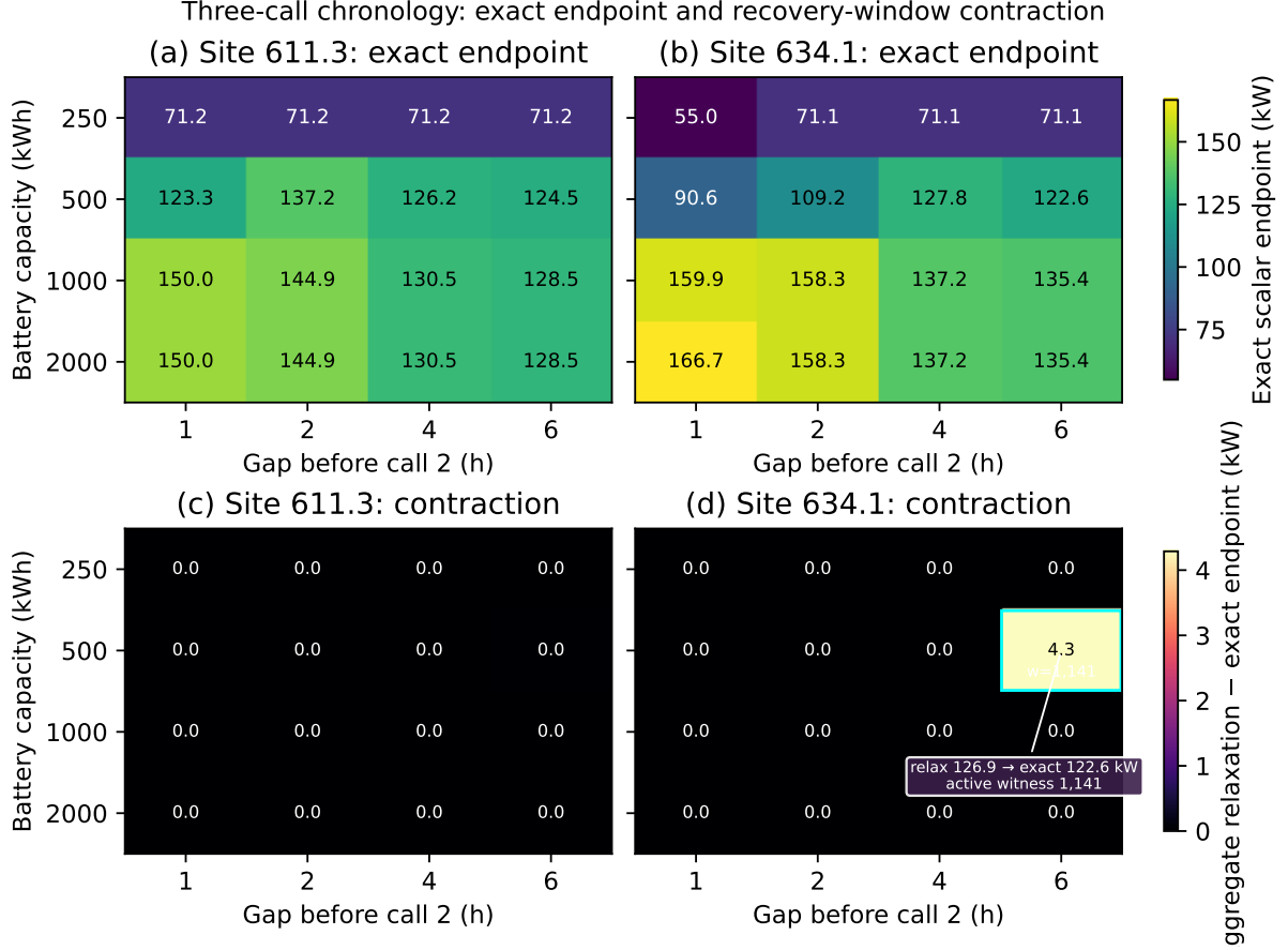
Figure 5: Predeclared three-call chronology stress under an always-visible terminal target. The top panels show exact scalar-LP endpoints across capacity and second-call gap at the two primary placements; the lower panels show the aggregate-relaxation minus exact endpoint contraction. The material 634.1, E = 500 kWh, 6-h cell is annotated with the paired relaxation/exact values and its 1,141 active cumulative-window witnesses.
