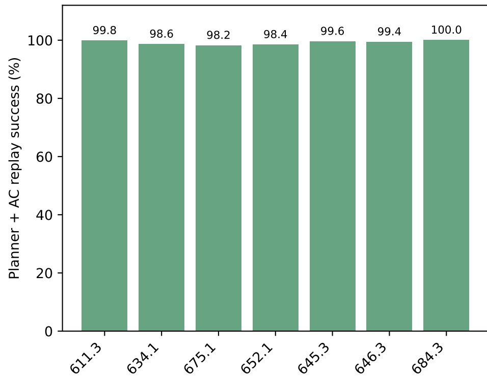
2013 fixed-offer evaluation
