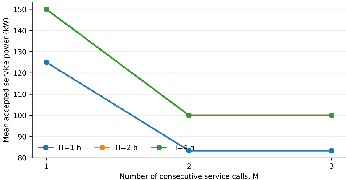
IEEE 123-node event-tree audit: sequence contraction
