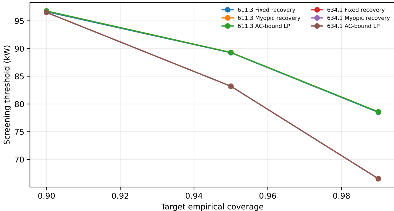
Descriptive empirical screening thresholds
