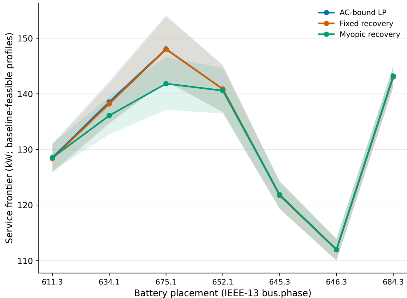
B. Repeated-service frontier by placement
