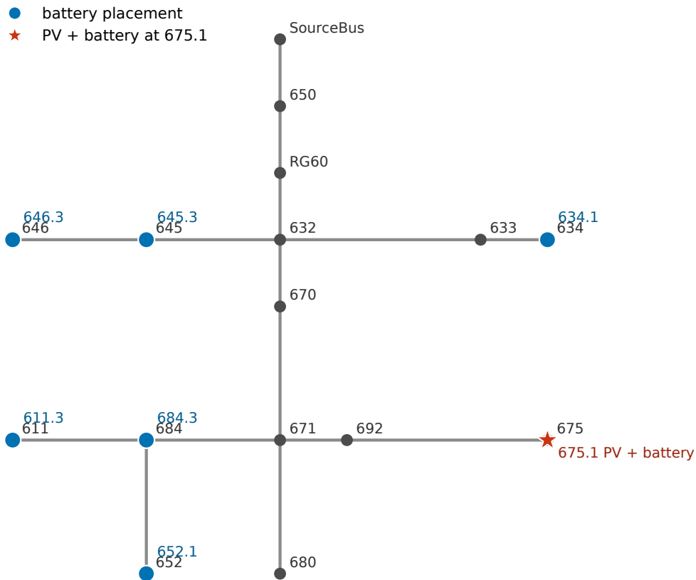
A. IEEE-13 placement set
