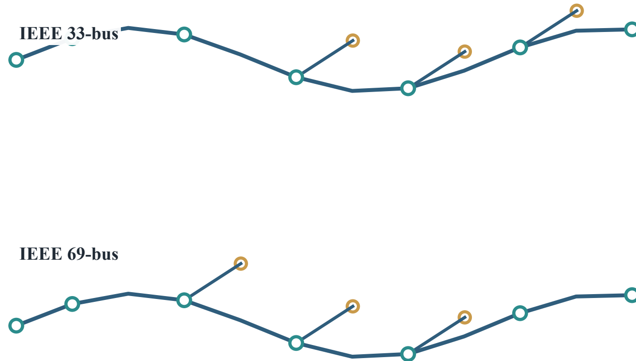
(a) Distribution feeders used in the study
