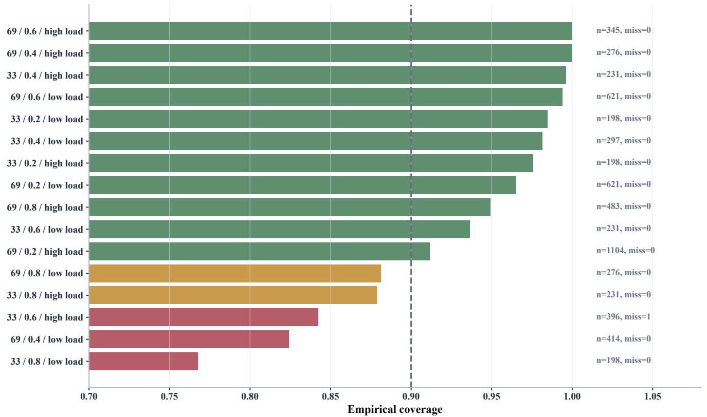
Figure 4: Per-family conditioned calibration audit. The bars show empirical coverage by topology/PV/loading family with sample counts and missed violations, exposing the small-family regimes where shrinkage matters.
