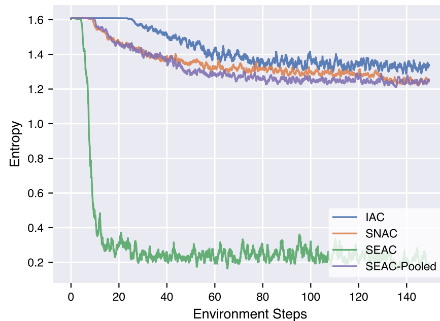
(e) small-4ag: Train Entropy
