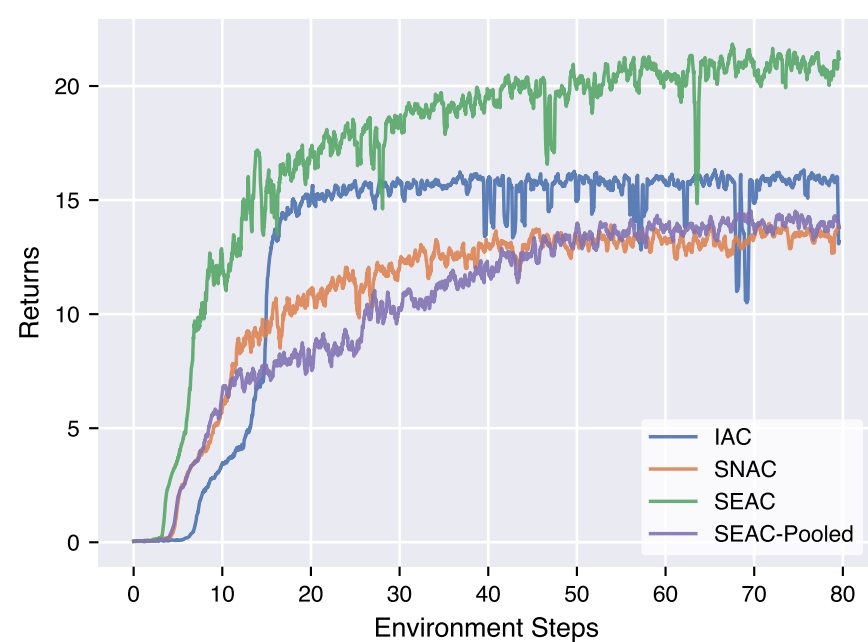
(a) tiny-2ag: Train Reward
