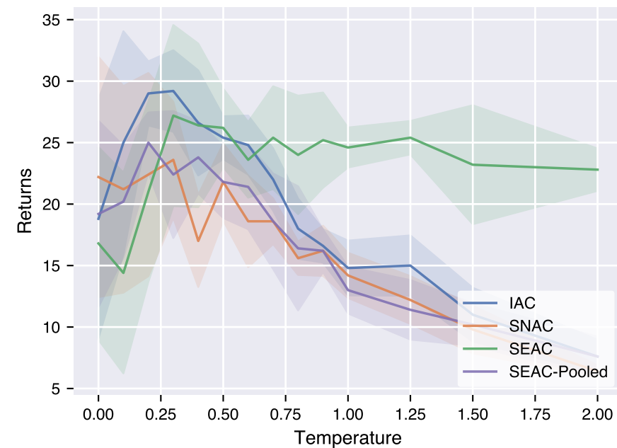
(f) small-4ag: Temperature Sweep
