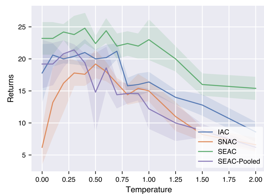
(c) tiny-2ag: Temperature Sweep
