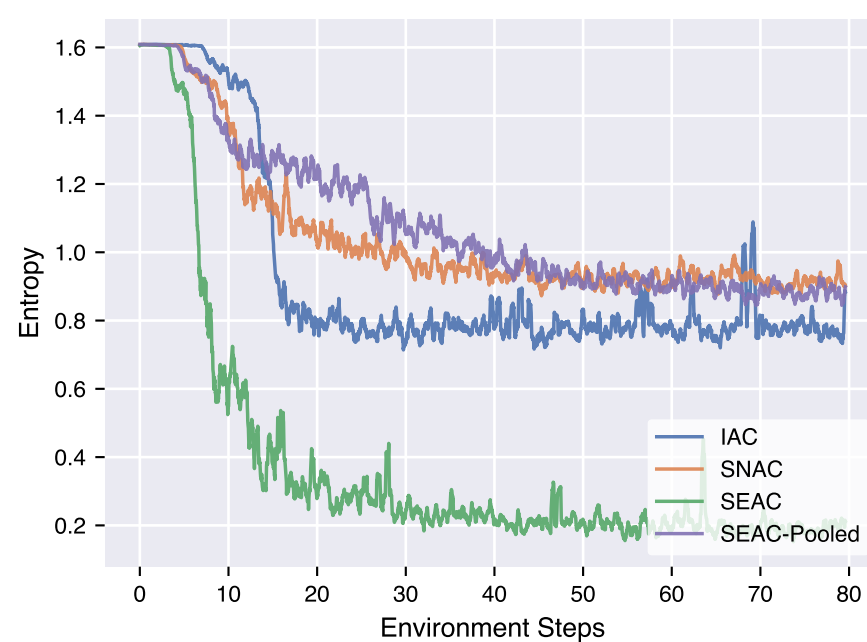
(b) tiny-2ag: Train Entropy
