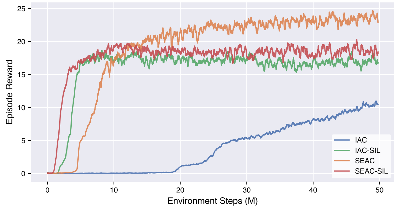
Small-4ag: SIL Convergence Comparison
