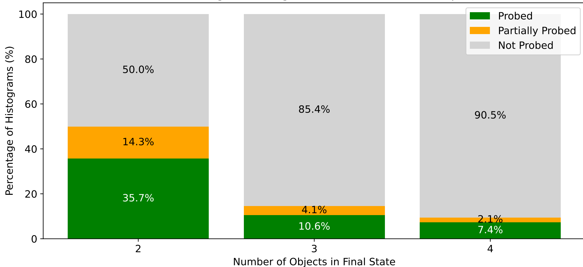
Percentage of Histograms Probed for Mass Bumps
