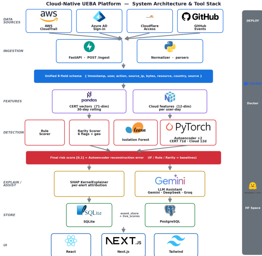
Fig. 1. Argus system architecture and tool stack: four cloud sources are normalised into one schema, scored by a label-free autoencoder with rarity and rule baselines, explained via SHAP and an LLM assistant, then surfaced on a web dashboard.
