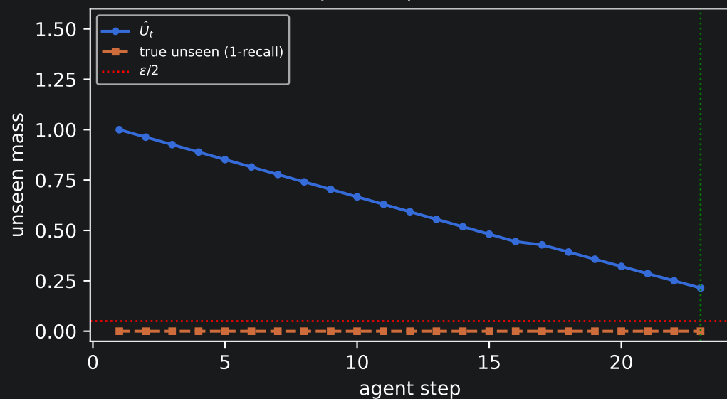
\varepsilon=0.1 : stop @ step 23, recall=100%
