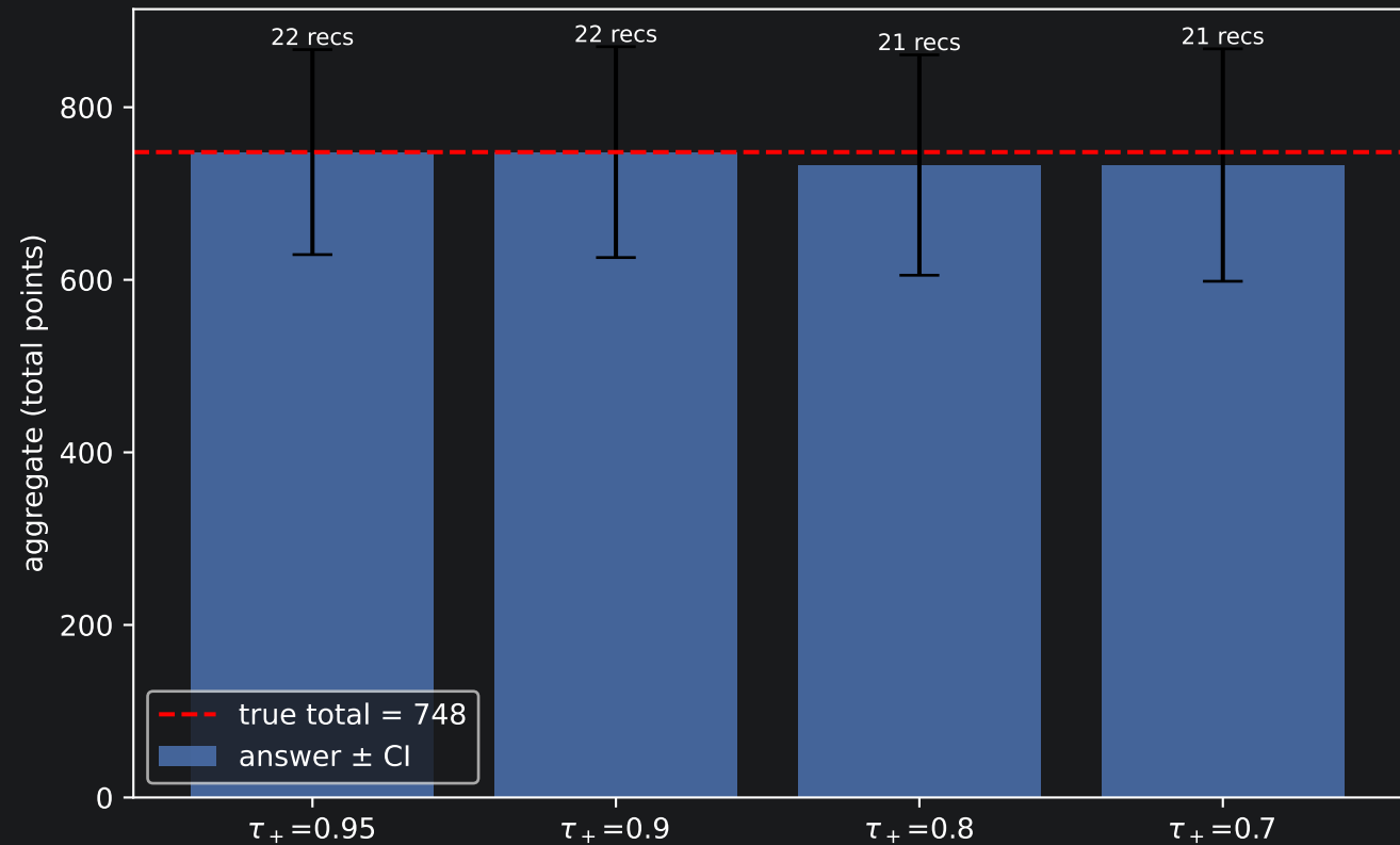
Exp 3: ER error propagation — CI coverage as the matcher is loosened
