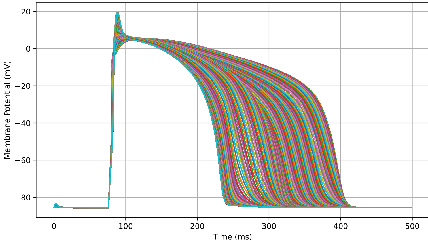
AP Traces sharpness=125.0000, width=266, amplitude=0.85
