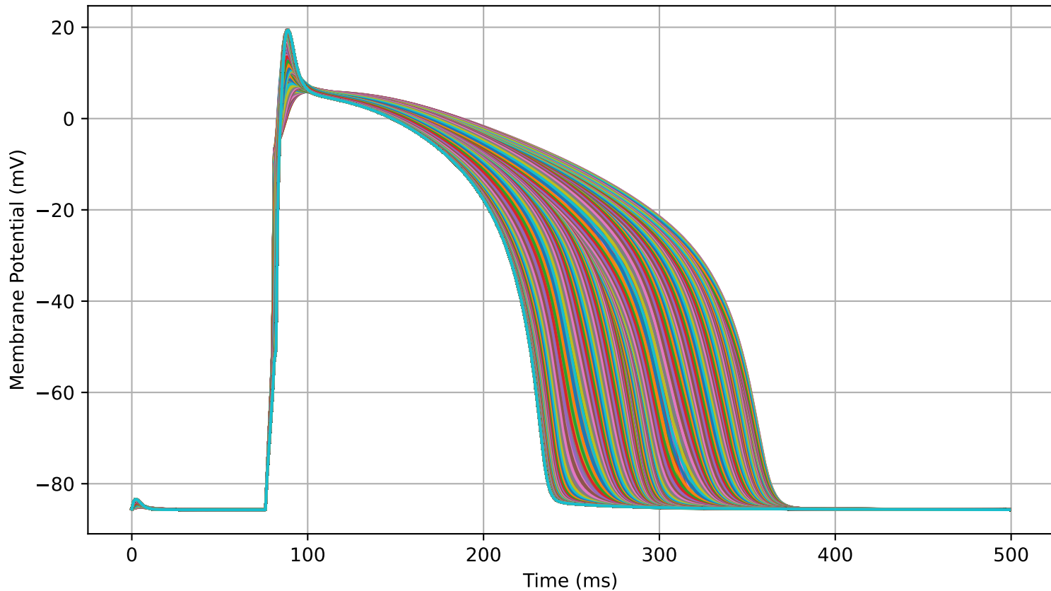
AP Traces sharpness=125.0000, width=266, amplitude=0.8
