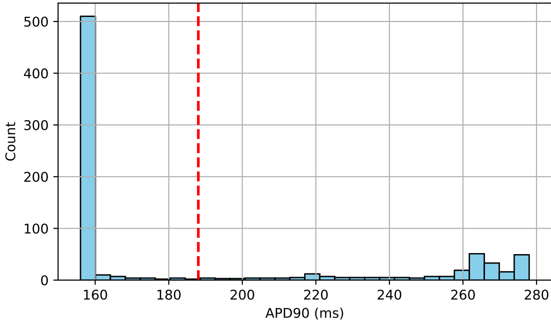
APD90 Distribution sharpness=125.0000, width=266, amplitude=0.83
