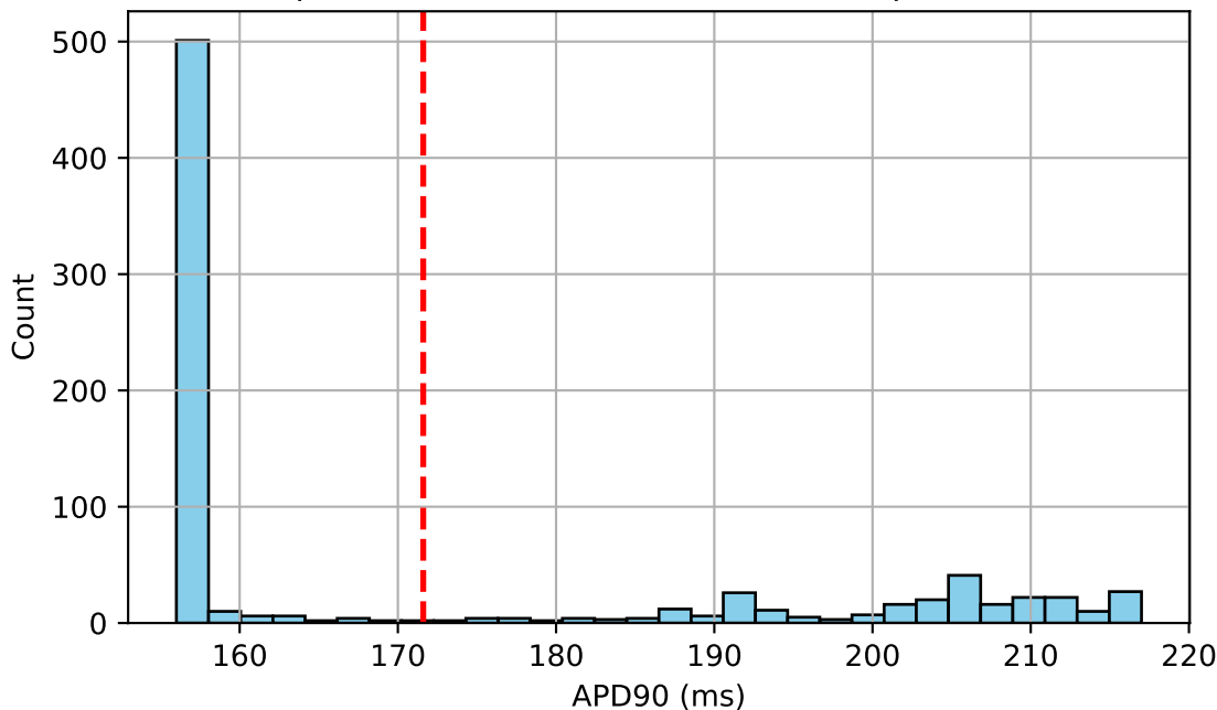
APD90 Distribution sharpness=125.0000, width=266, amplitude=0.6
