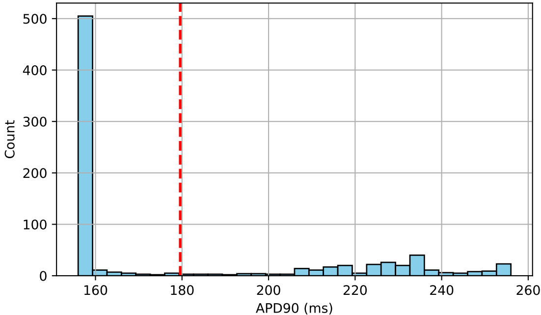
APD90 Distribution sharpness=125.0000, width=266, amplitude=0.7
