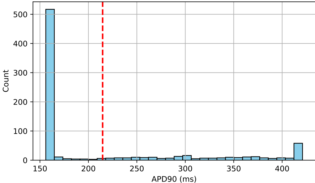
APD90 Distribution sharpness=125.0000, width=266, amplitude=0.9
