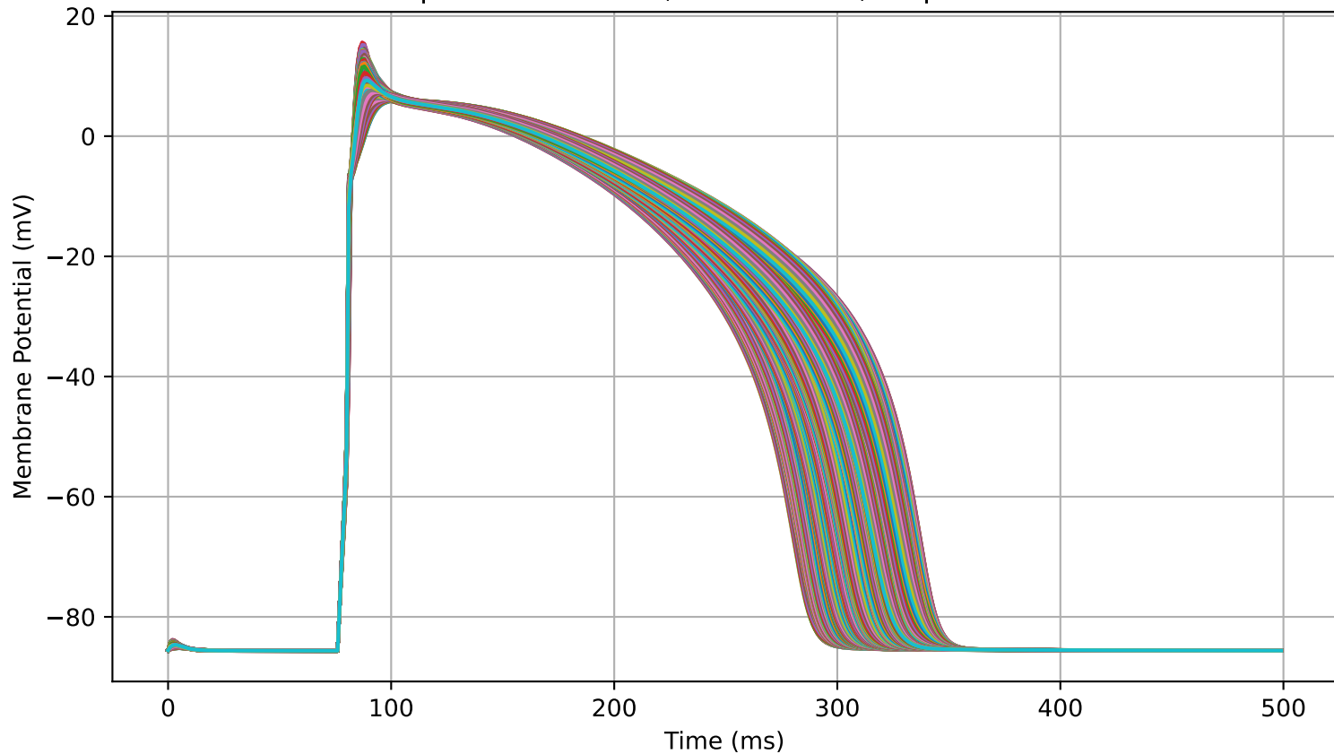
AP Traces sharpness=125.0000, width=1600, amplitude=0.7
