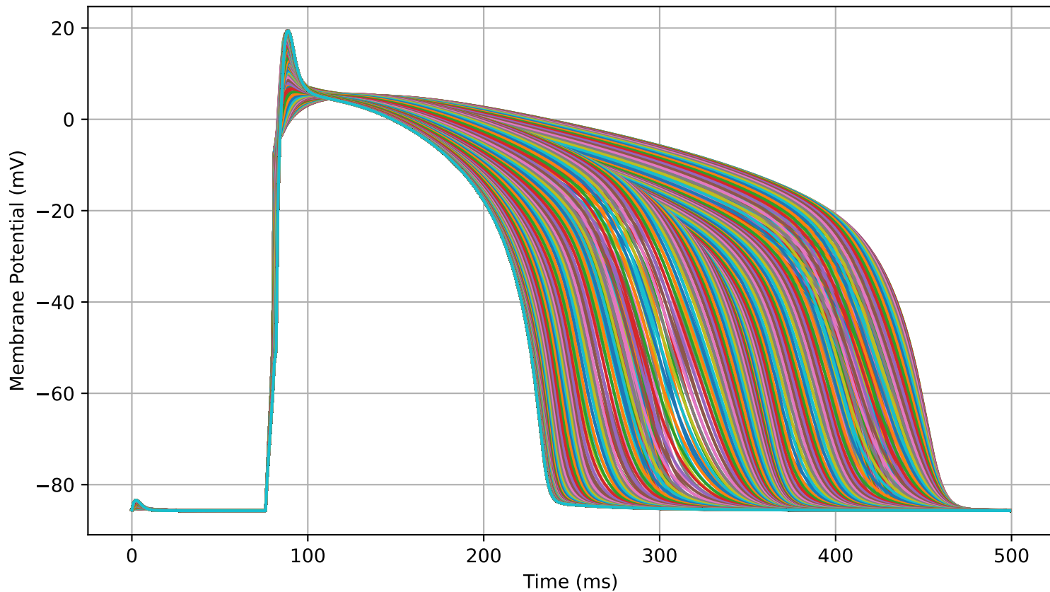
AP Traces sharpness=0.1250, width=266, amplitude=0.89
