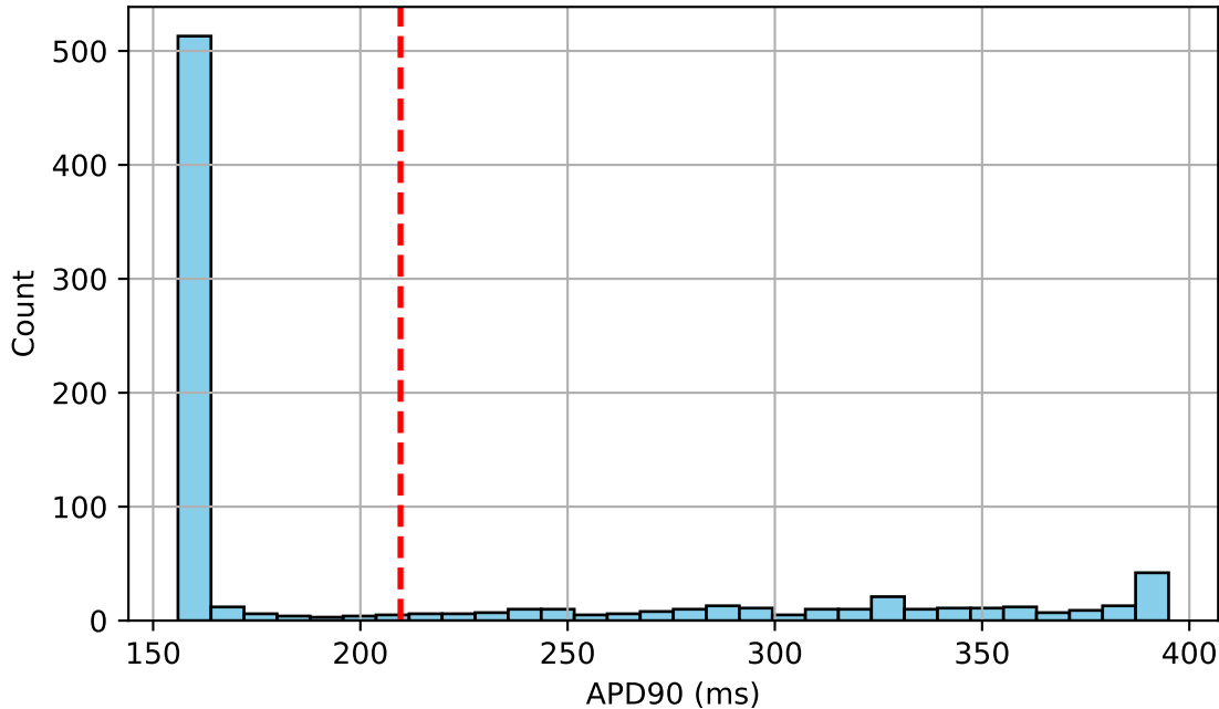
APD90 Distribution sharpness=62.5000, width=266, amplitude=0.89
