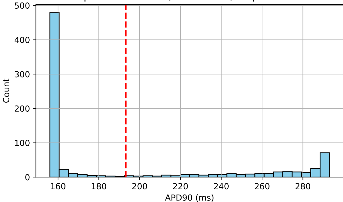
APD90 Distribution sharpness=125.0000, width=266, amplitude=0.89
