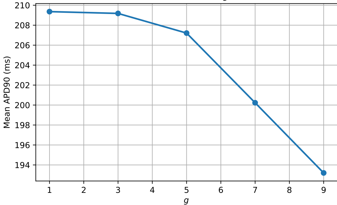
Mean APD90 vs g
