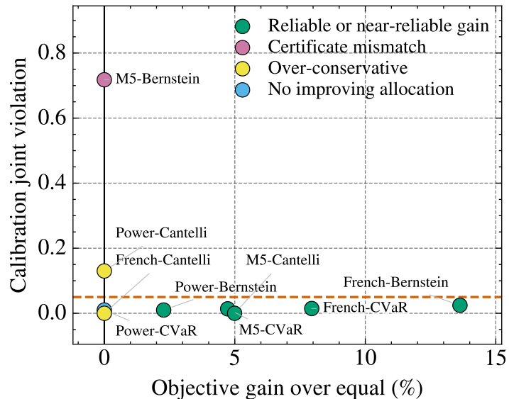
In-sample
