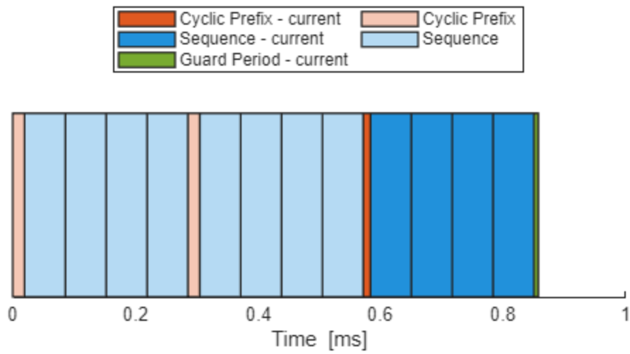
Time-Domain Structure of PRACH Preamble Format A2/B2 within One 15 kHz Carrier Slot (NPRACHSlot = 0)
