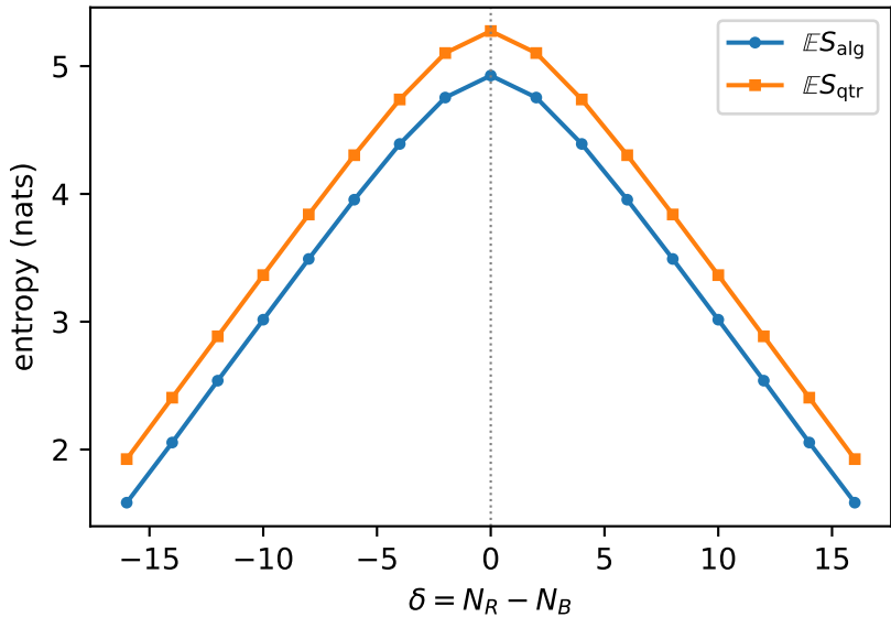
Page curves ( N = 24 )
