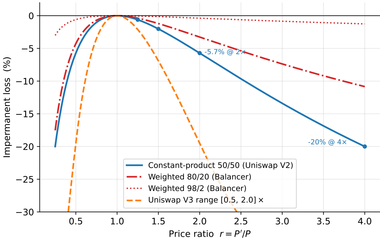
Impermanent loss vs price divergence
