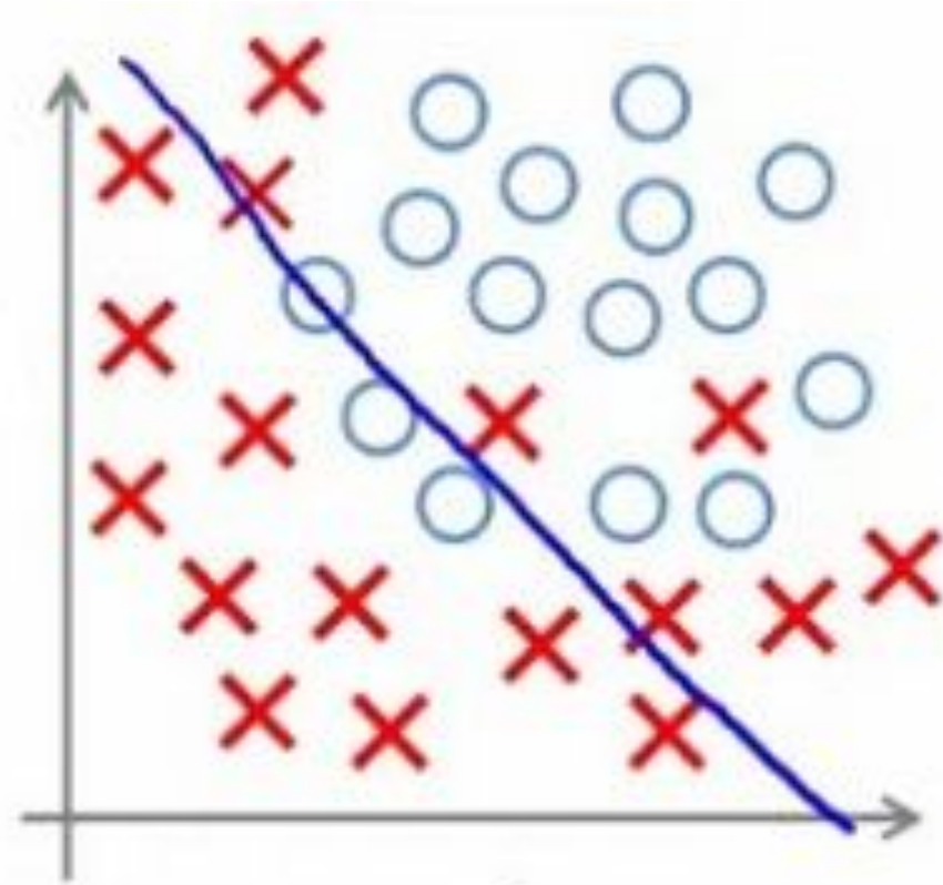
Under-fitting
