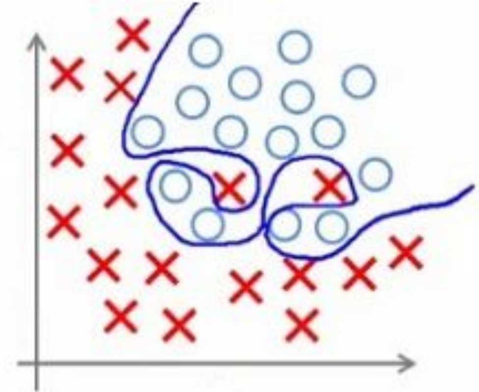
Over-fitting
