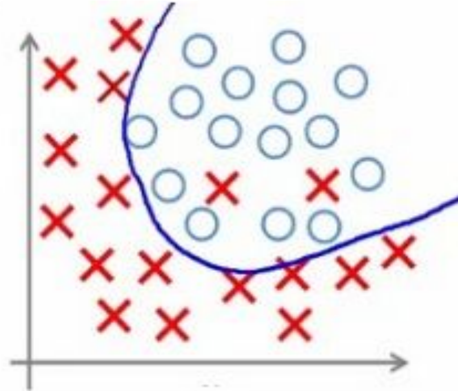
Appropriate-fitting
