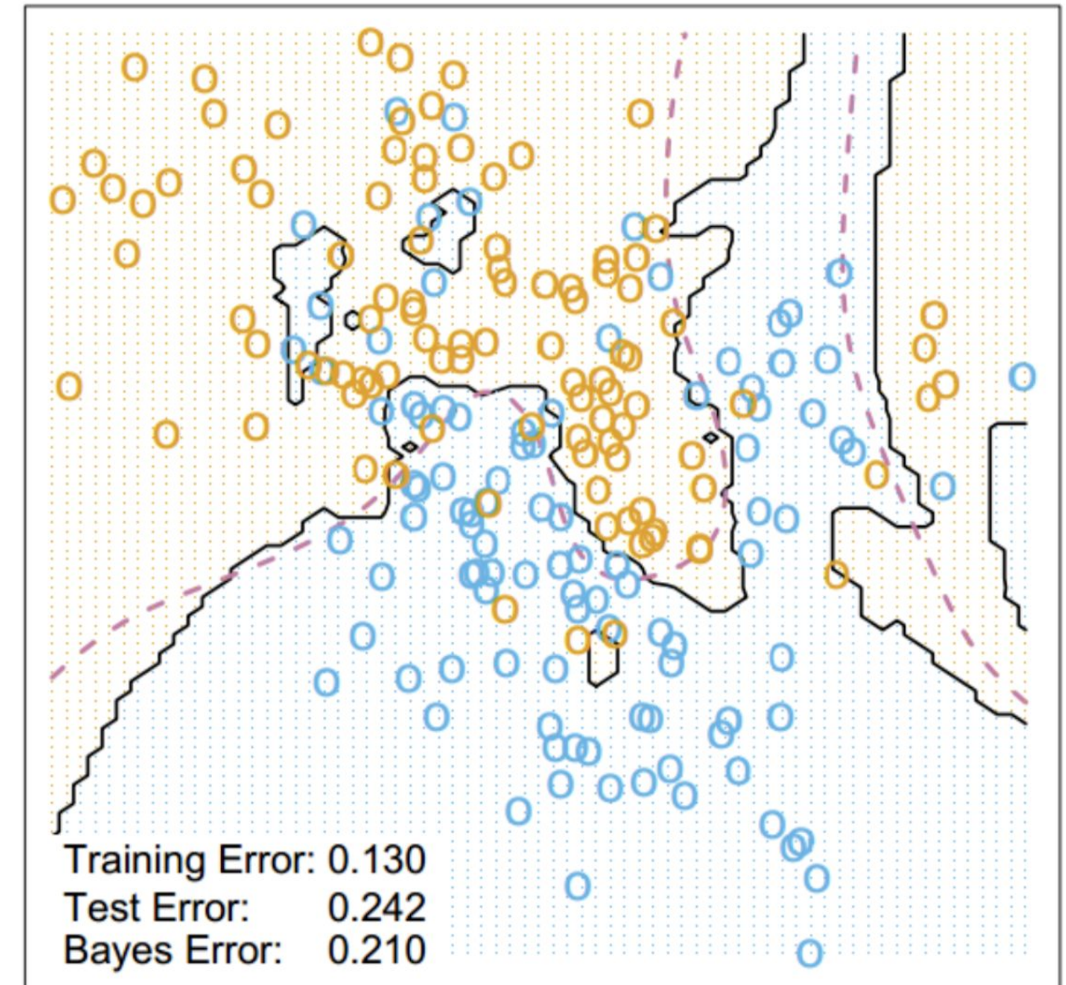
3-Nearest Neighbors
