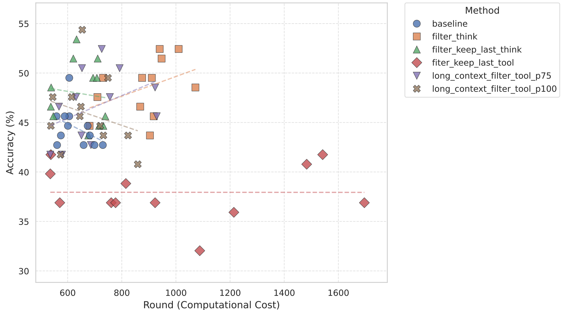
Accuracy vs. Round Consumption by Agent Strategy
