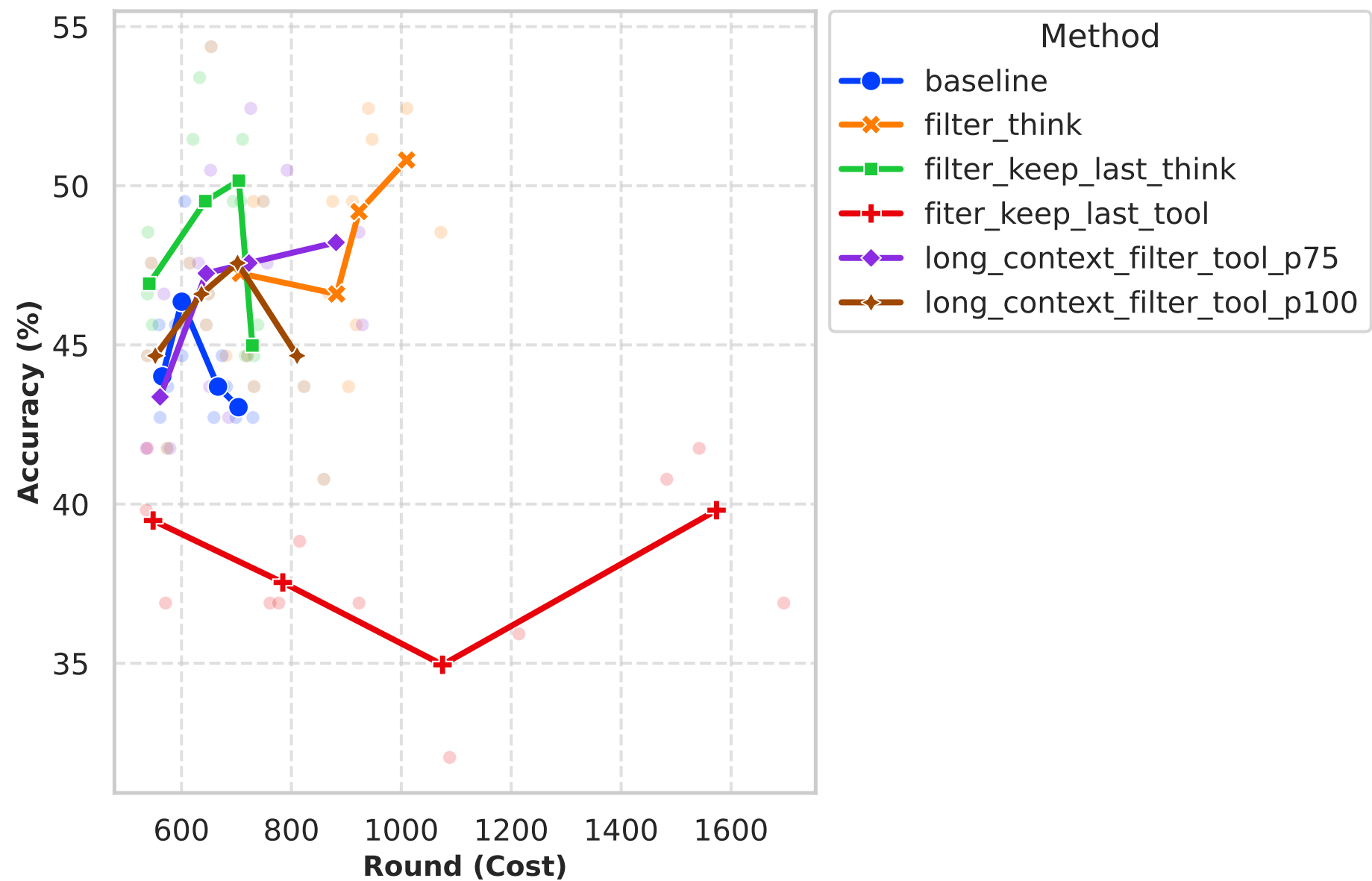
Summary: Scaling Law Comparison Across Methods
