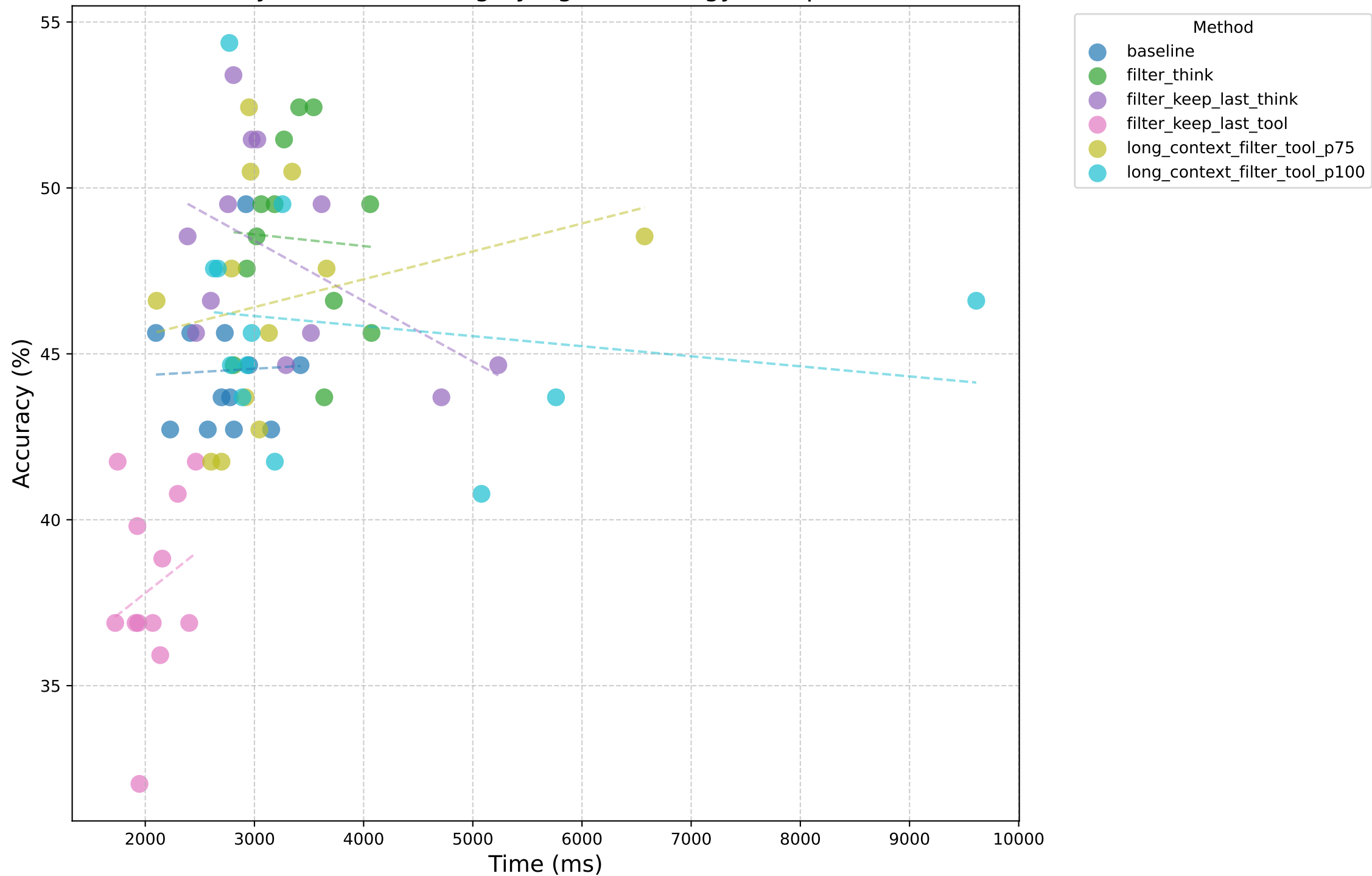
Accuracy vs. Time Scaling by Agent Strategy (DeepSeek V3)
