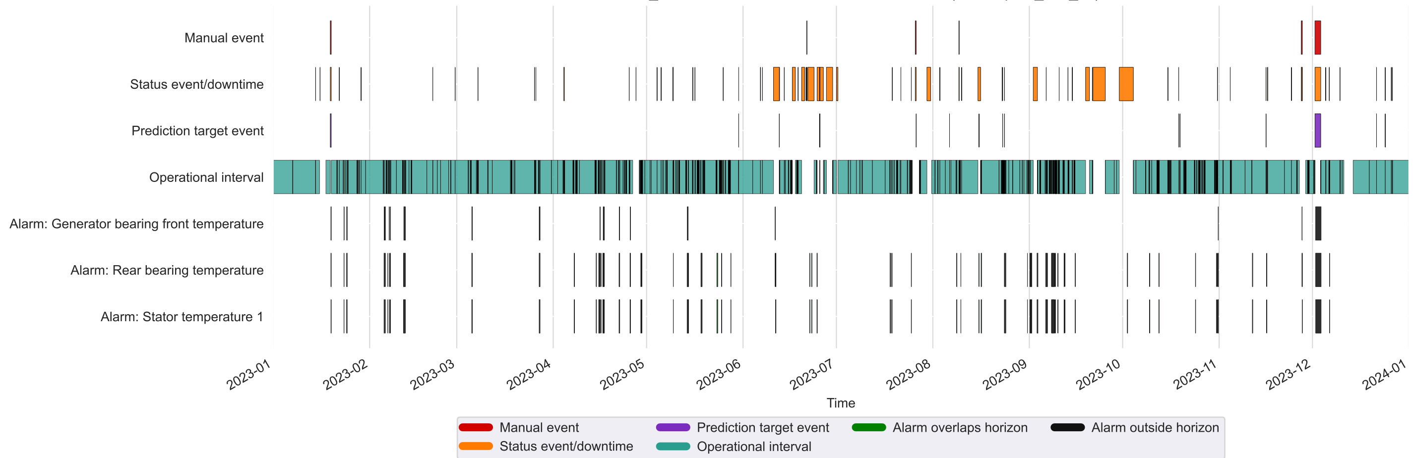
Kelmarsh_1: labelled intervals and detection alarms (2023, q995_c12_v2)
