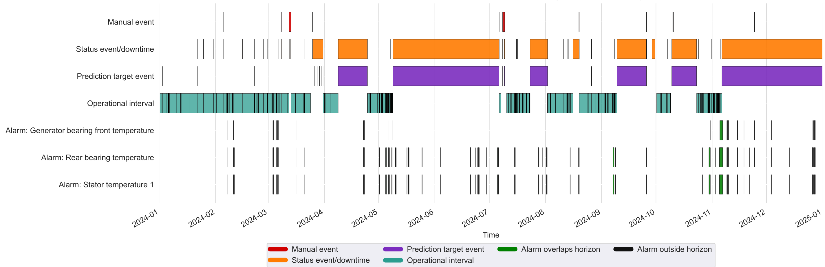
Kelmarsh_1: labelled intervals and detection alarms (2024, q995_c12_v2)
