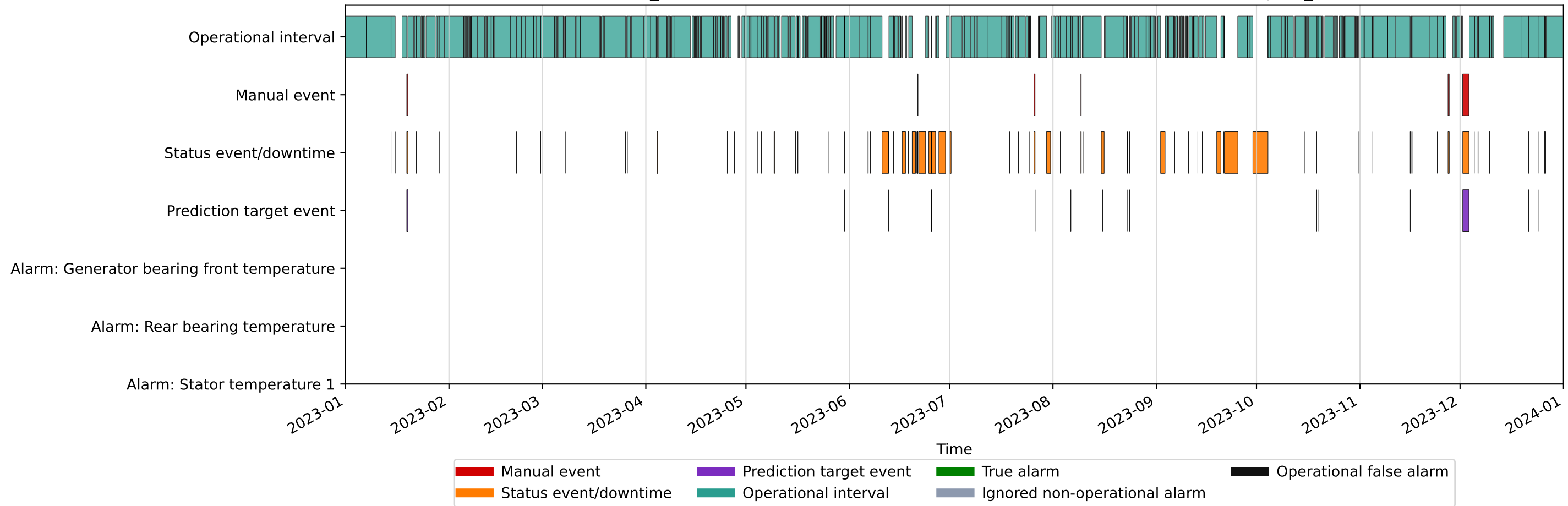
Kelmarsh_1: labelled intervals and detection alarms (2023, Residual baseline, q995_c6)
