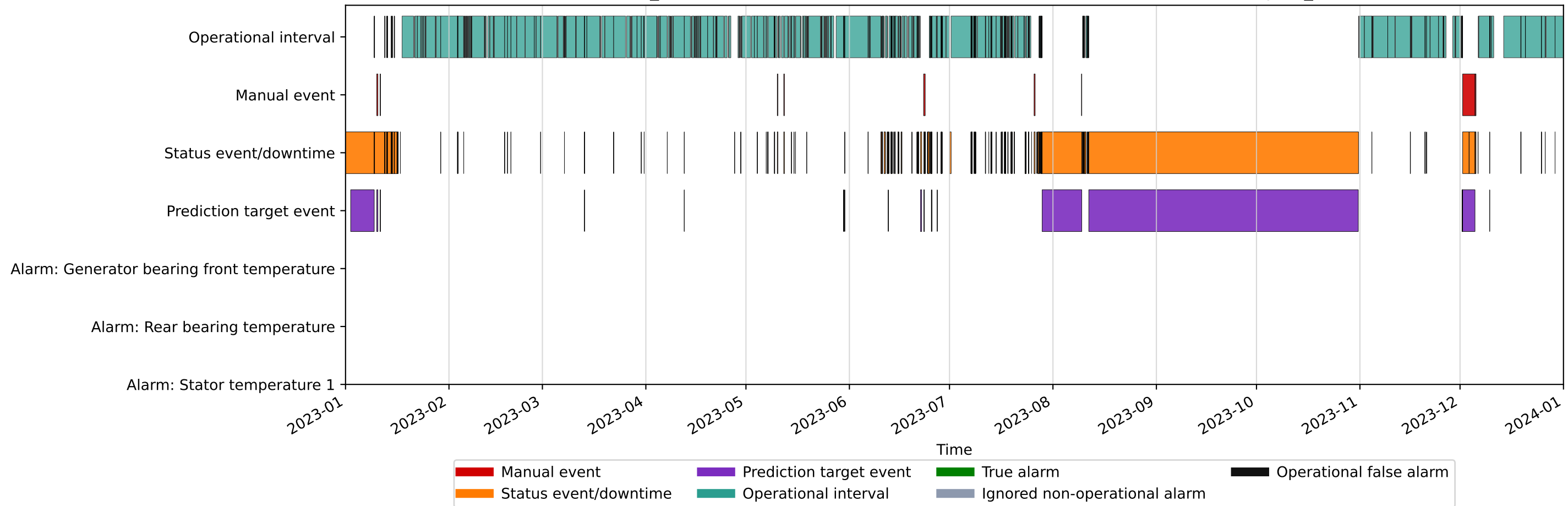
Kelmarsh_2: labelled intervals and detection alarms (2023, Residual baseline, q995_c6)
