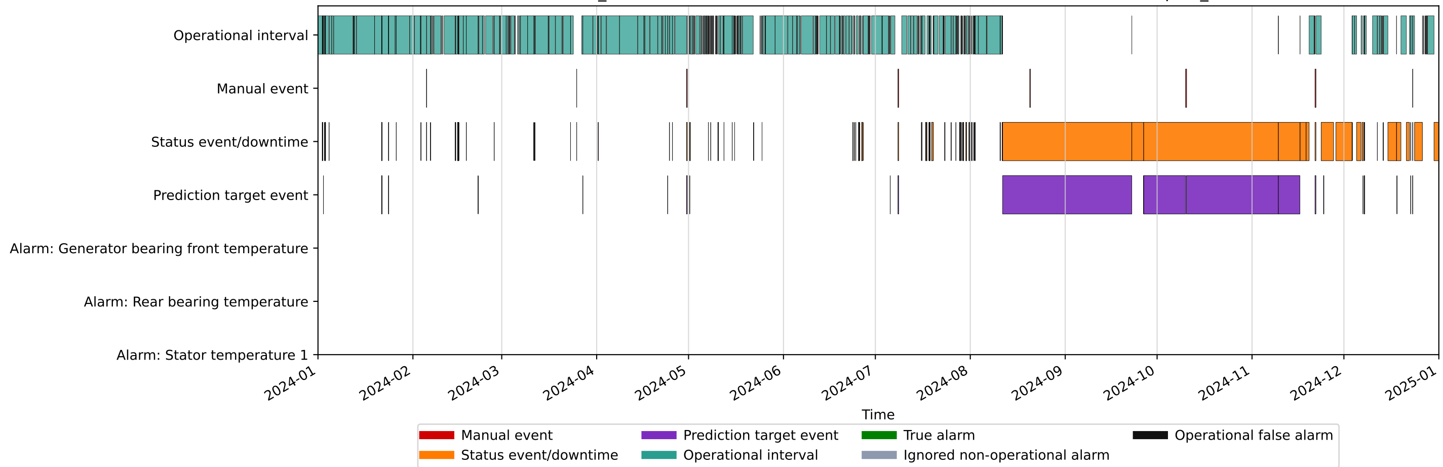
Kelmarsh_2: labelled intervals and detection alarms (2024, Residual baseline, q995_c6)
