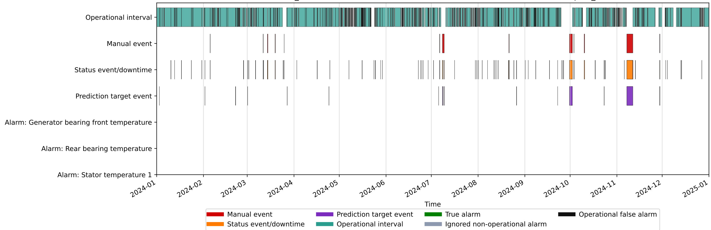
Kelmarsh_3: labelled intervals and detection alarms (2024, Residual baseline, q995_c6)
