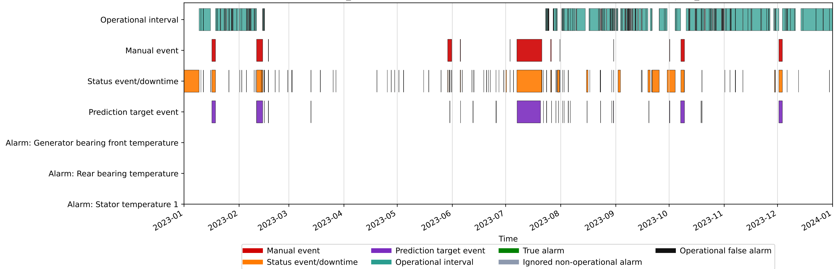
Kelmarsh_4: labelled intervals and detection alarms (2023, Residual baseline, q995_c6)
