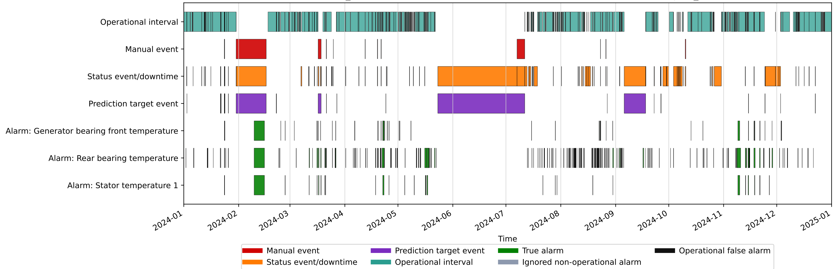
Kelmarsh_4: labelled intervals and detection alarms (2024, Residual baseline, q995_c6)
