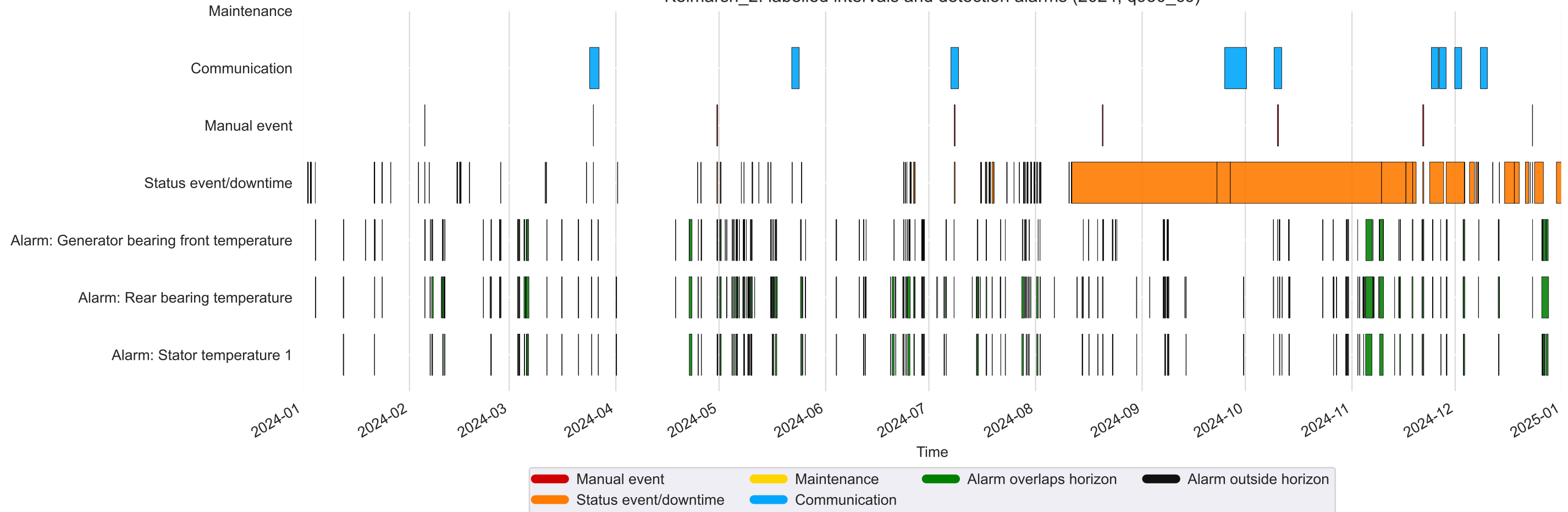
Kelmarsh_2: labelled intervals and detection alarms (2024, q950_c6)
