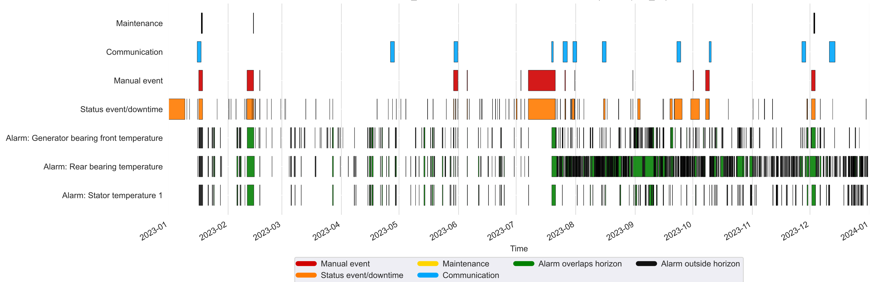
Kelmarsh_4: labelled intervals and detection alarms (2023, q950_c6)
