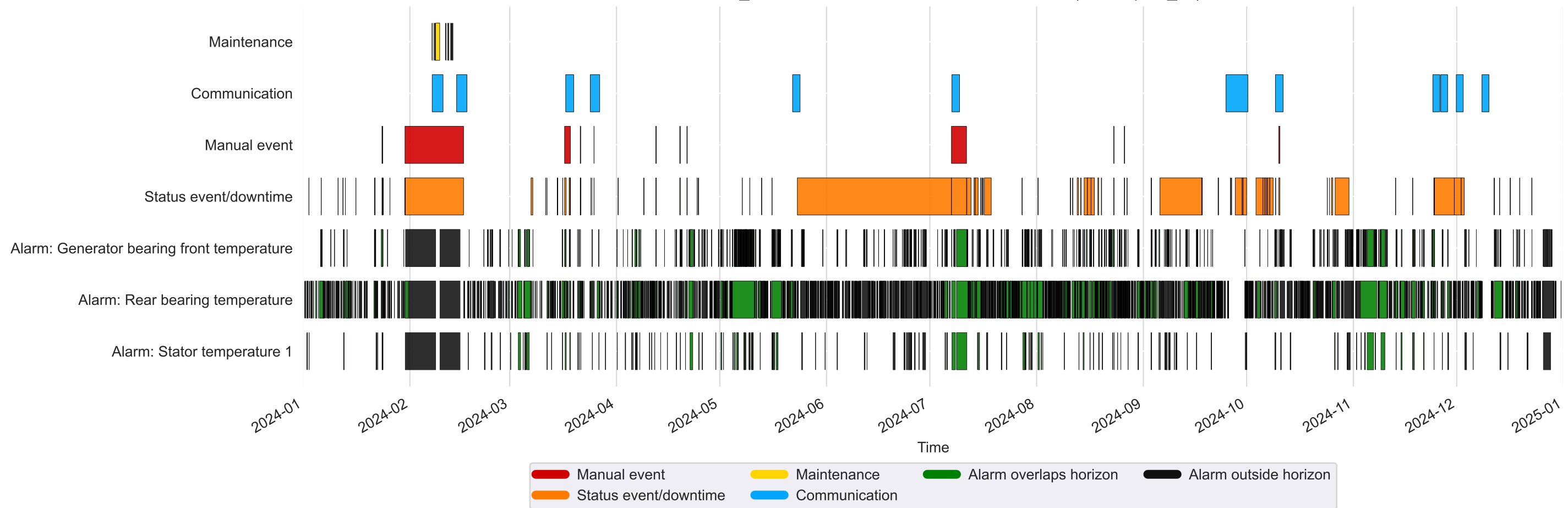
Kelmarsh_4: labelled intervals and detection alarms (2024, q950_c6)
